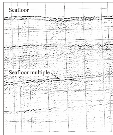
Plate 6: Sub bottom profiler line 08.
