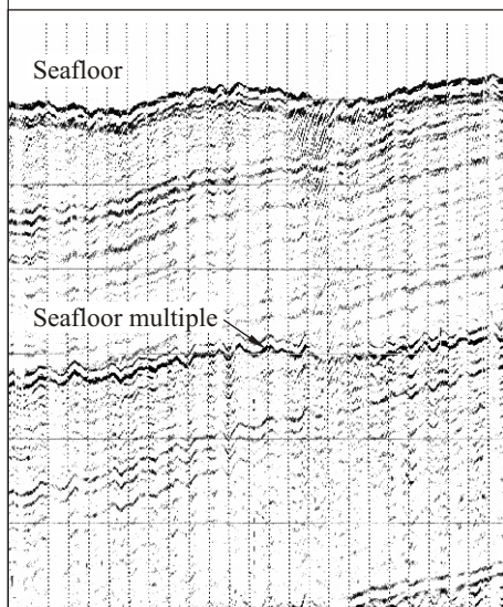
Plate 5: Sub bottom profiler line 07.
