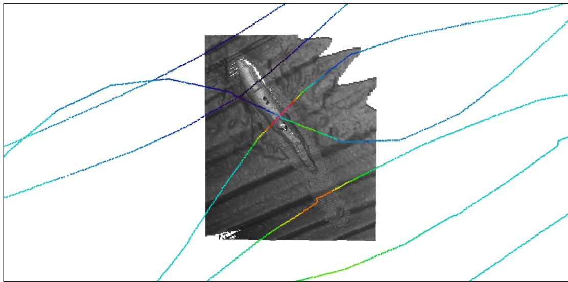
Plate 1: Magnetometer lines over multibeam sonar image.
