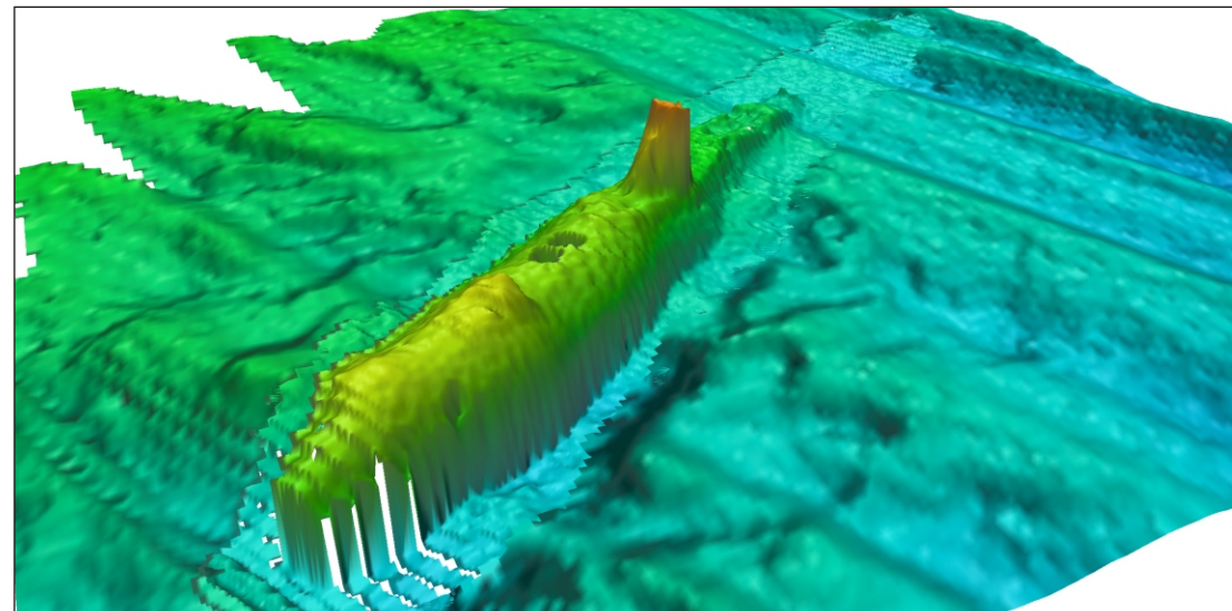
Plate 4: Multibeam image of HMS A1 , looking south.
