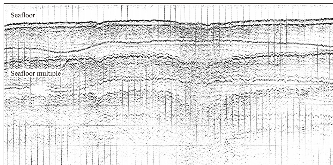
Plate 6: Sub bottom profiler line H70.
