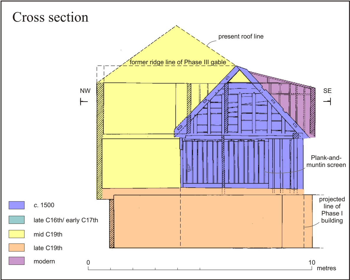
Fig. 2 Cross section through centre of building
