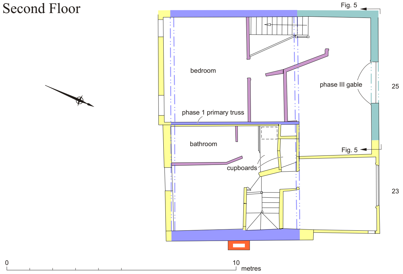
Fig. 4 First and second floor phase plans with inferred position of former walls.
