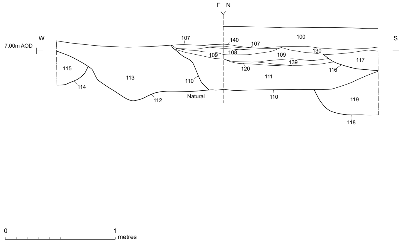
Fig. 13: Section 4 (1:20)
