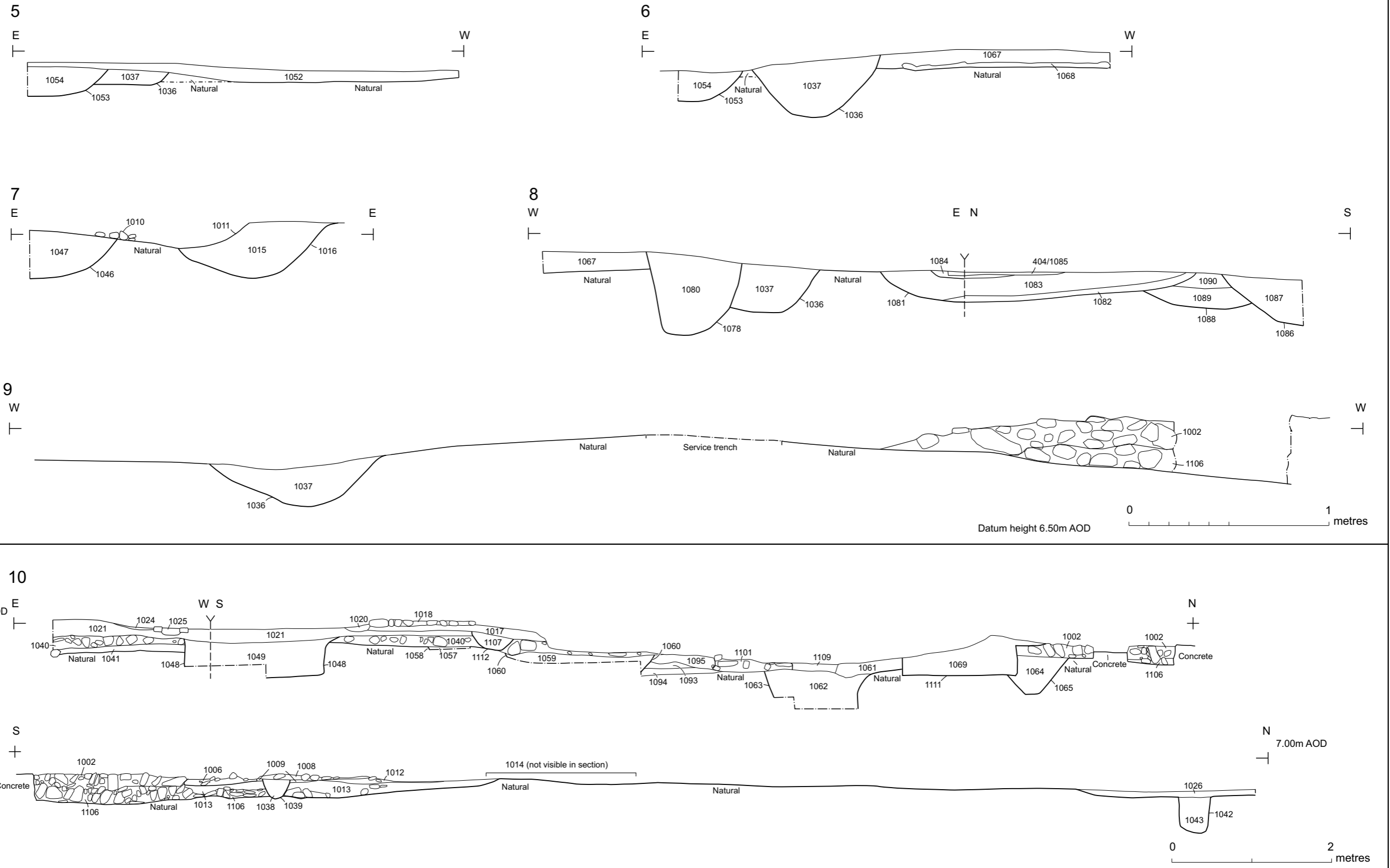
Fig. 14: Sections 5-9 (1:20) and 10 (1:50)
