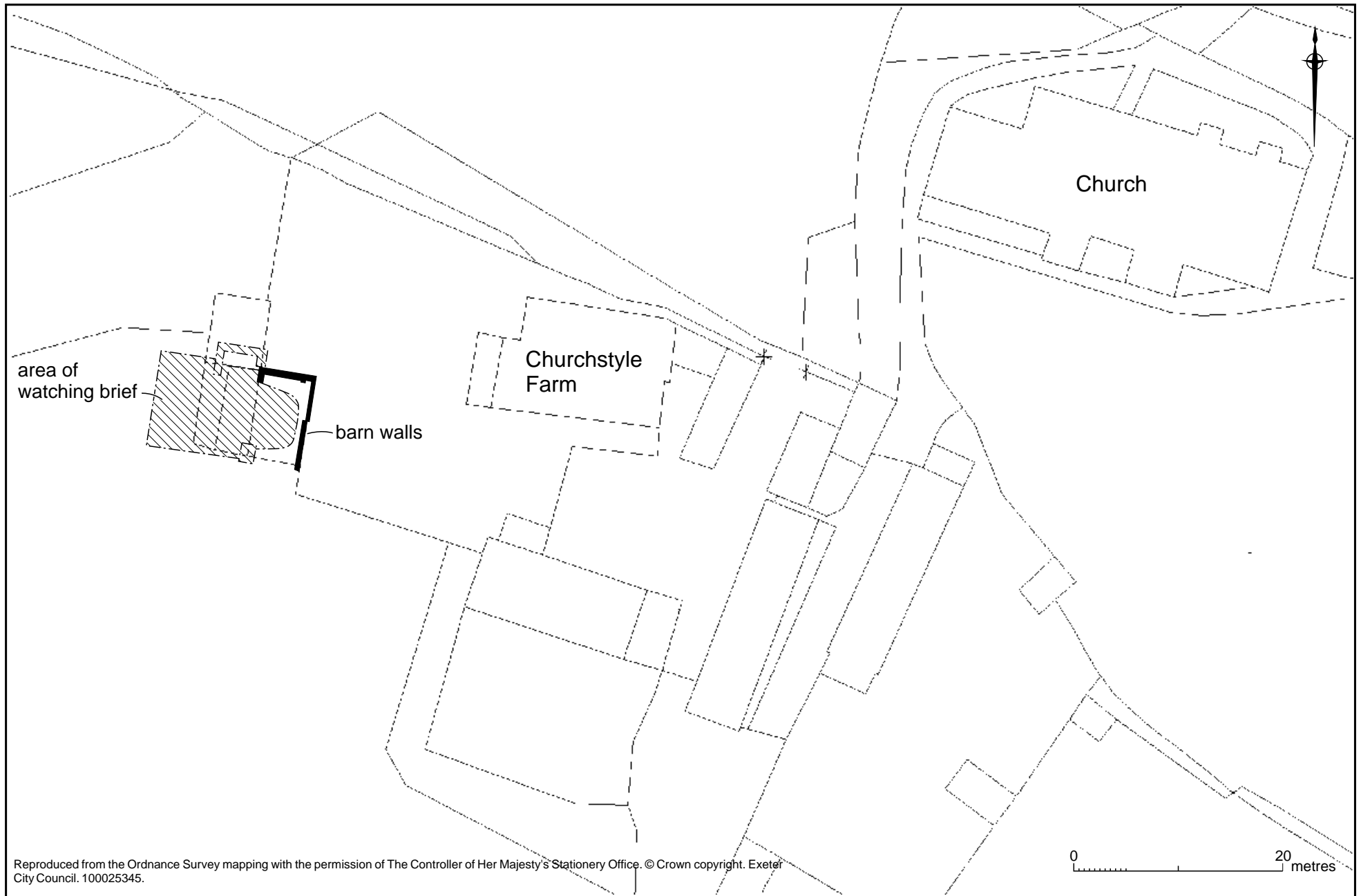
Fig. 1 Location plan (1:500)
