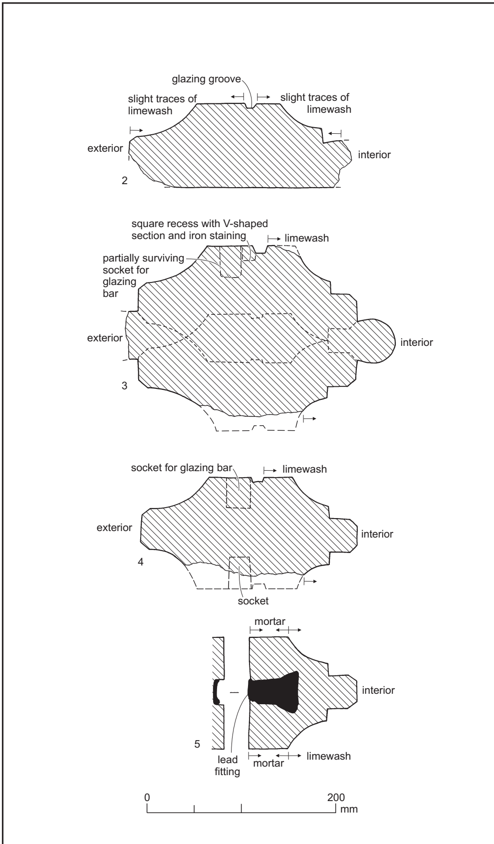
Fig. 4 Window mullions from Tedburn St Mary churchyard. Scale 1:4.
