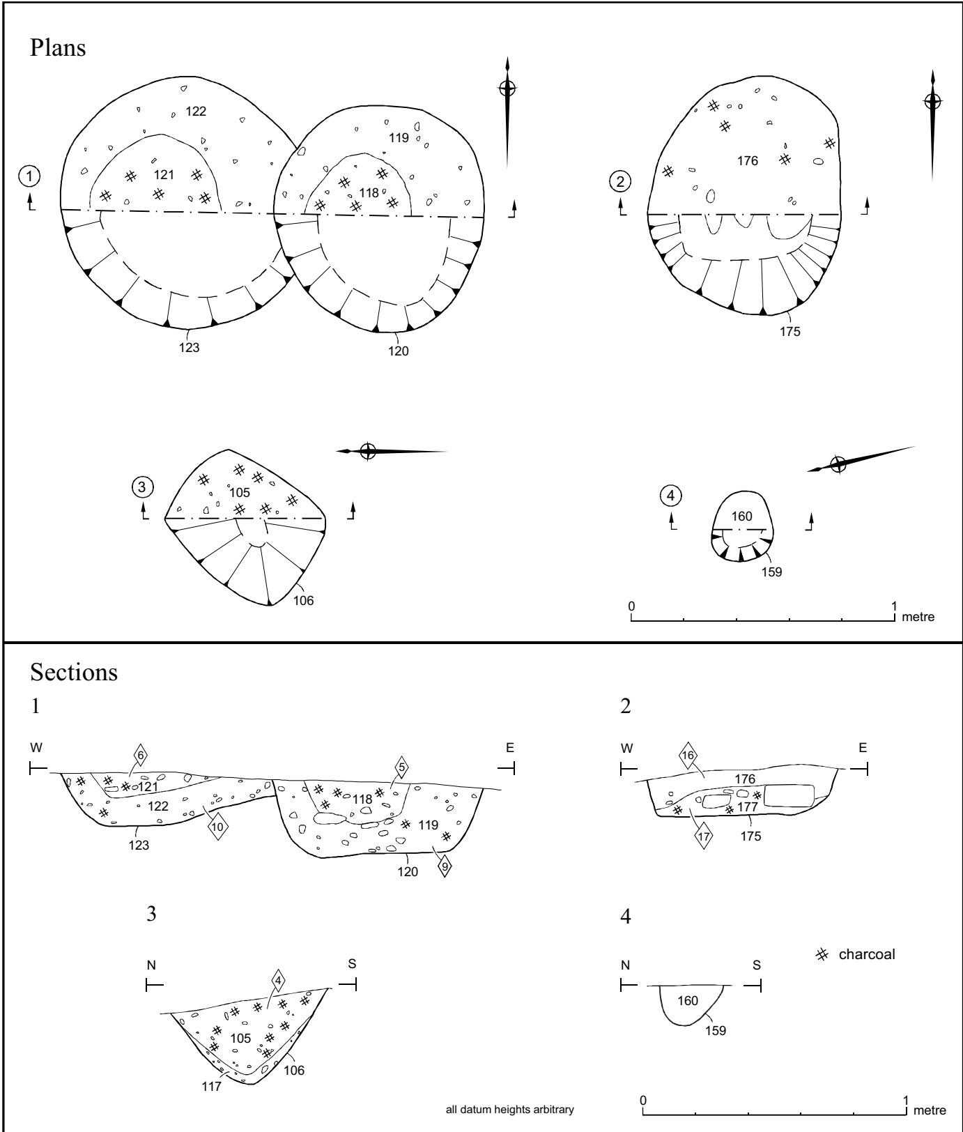
Fig. 5 Plans, and Sections through pits and post-holes. Scale 1:20.
