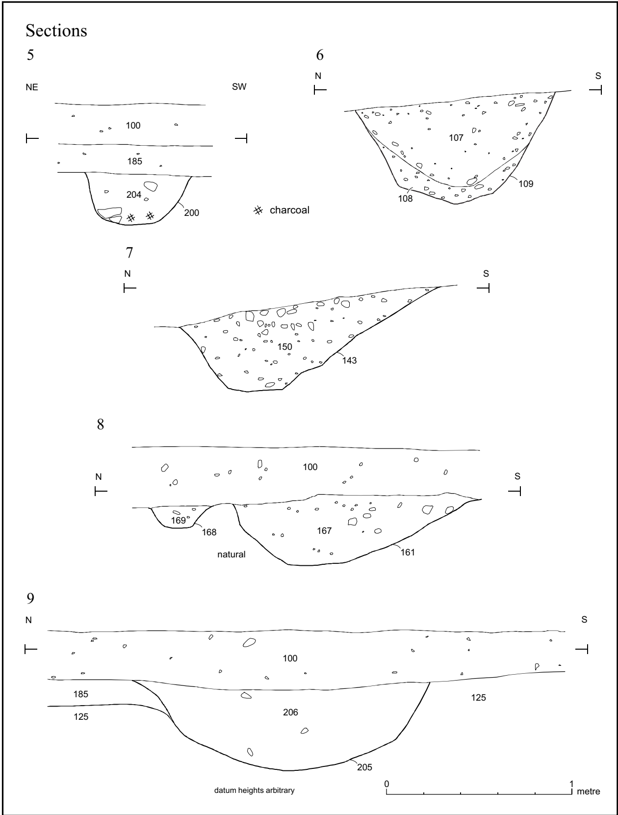
Fig 6 Sections through ditches. Scale 1:20.
