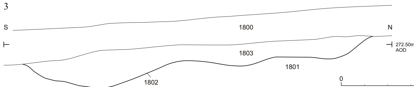
Fig. 8 Plans and sections.
