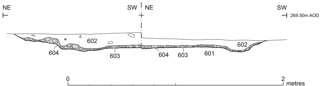
Fig. 7 Plans and sections.
