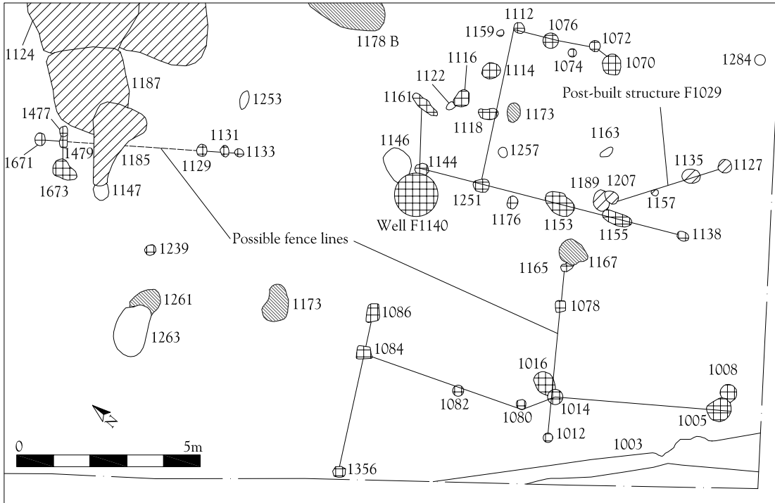
Figure 7 Plan of post-built structures and fence lines
