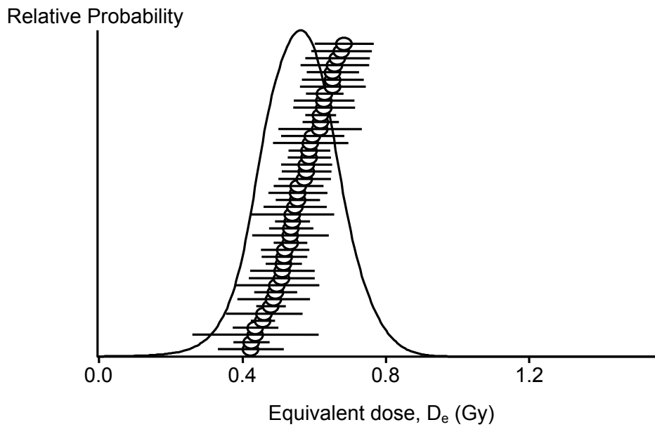
Figure 12: The distribution of D_e values obtained for a sample where a large number of aliquots were measured, namely sample 73BH-10/1. The 44 aliquots shown here in this probability density plot, clearly demonstrate that this sample is normally distributed, as are all of the samples in this OSL dating study.
