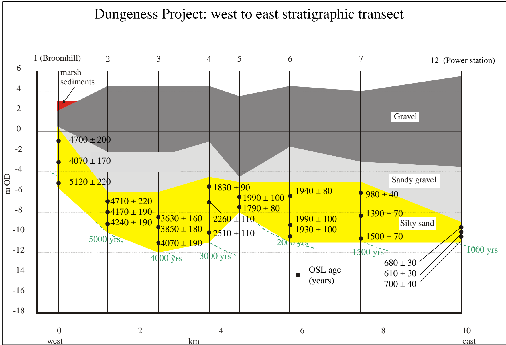
Figure 16a: Hypothetical isochrons (dotted lines) linking OSL ages for samples from the west – east stratigraphic transect across the Dungeness Foreland.
