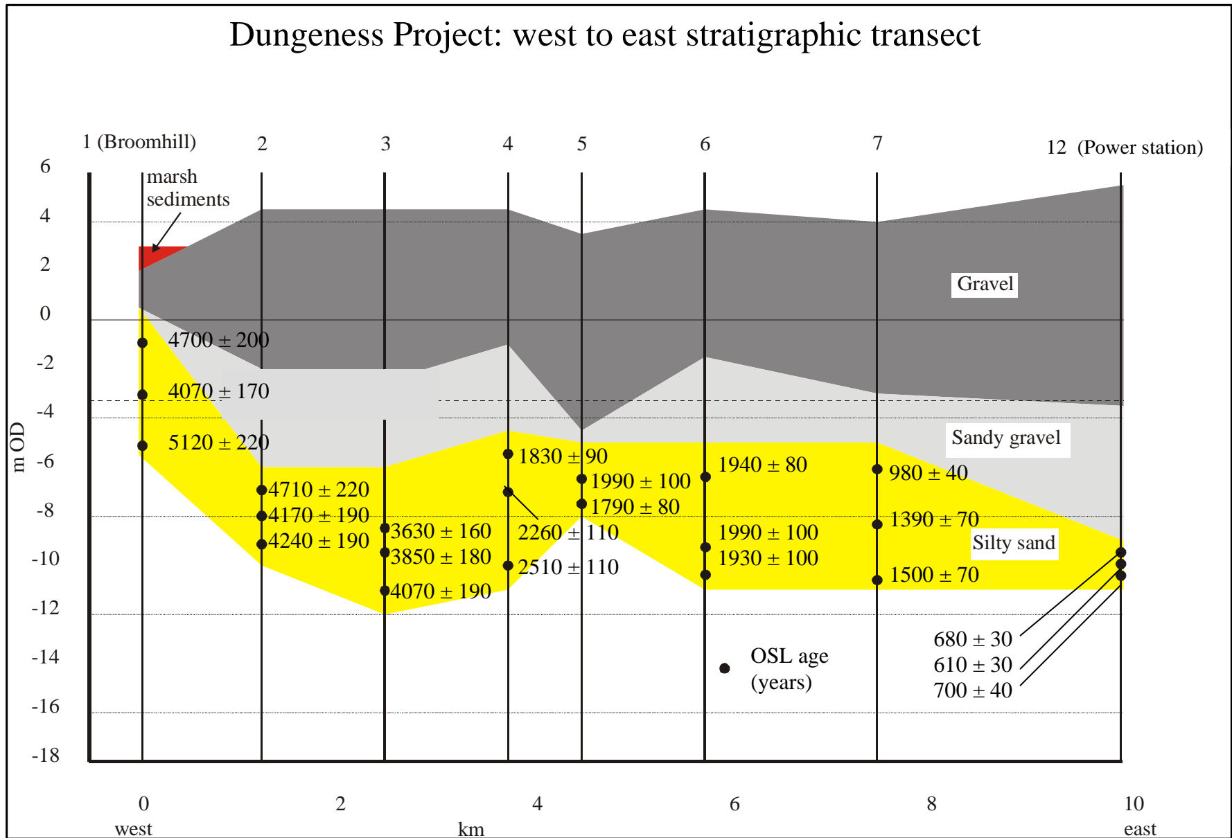
Figure 15a: OSL ages of samples from the west – east stratigraphic transect across the Dungeness Foreland.
