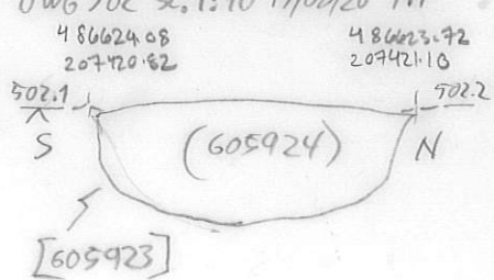
NE FAC. SECT. POST HOLE [605923] DWG 502 SCL. 1:10 17/08/20 FA
