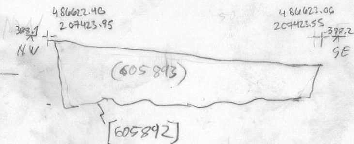
W FAC. SECT. POST HOLE [605892] DWG 388 SCL. 1:10 14/08/20 FA
