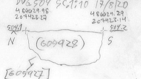
SW FAC. SECT. POST HOLE [605927] DWG 504 SCL. 1:10 17/08/20 FA
