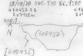
W FAC. SECT. POST HOLE [605936] DWG 508 SCL. 1:10 18/08/20 FA
