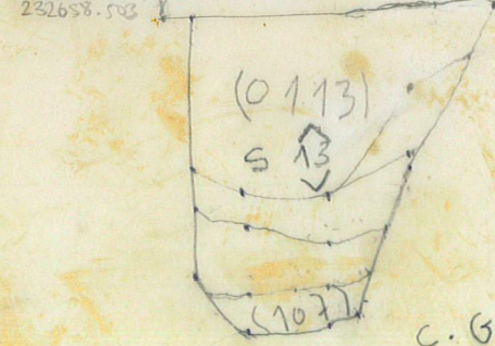
DWG 33 1:10 07-01-2021 East Face Posthole [00106] om 5/1/21 1:10
