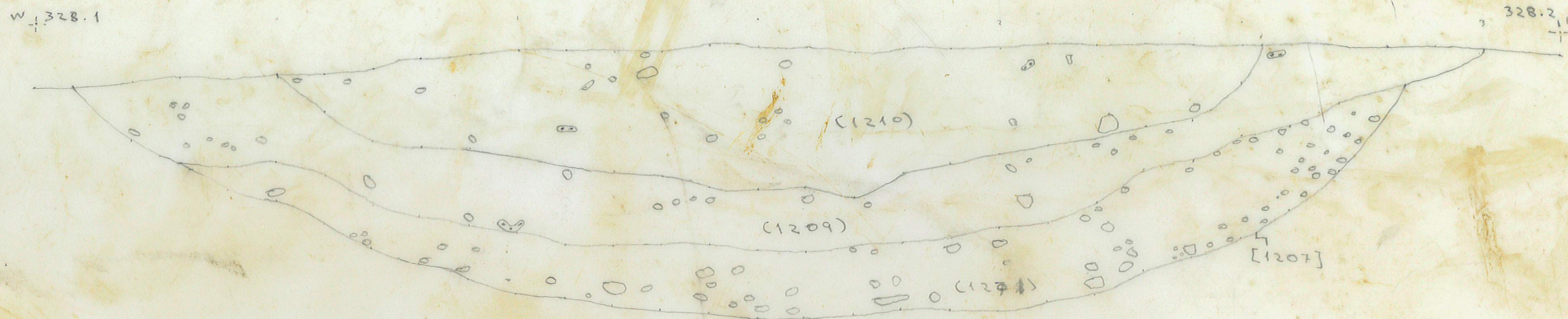
S FACING SECTION OF PIT [1207] DWG H 328 NL 8-7-21 1:10 C25120
