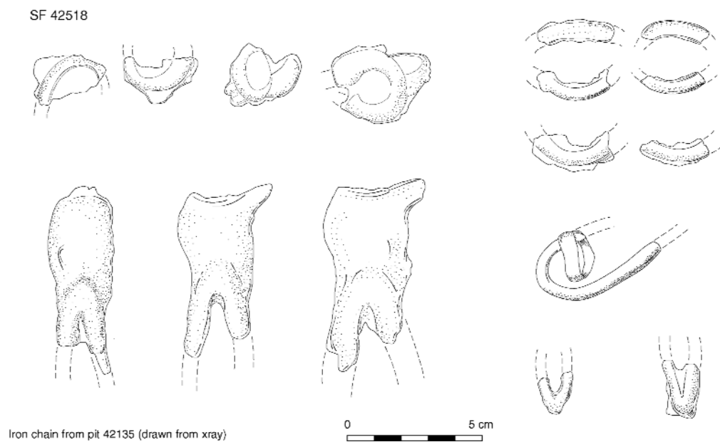
FIGURE 12 Metalwork from Plot 4.02. Scale 1:1 and 1:2
