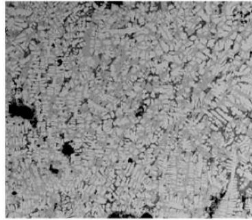
No. 4: Backscattered electron image of the microstructure of furnace slag specimen C2. The microstructure features the same mineral phases as the previous three specimens shown above, although the higher proportion of the iron oxide phase (wustite) is noticeable.
