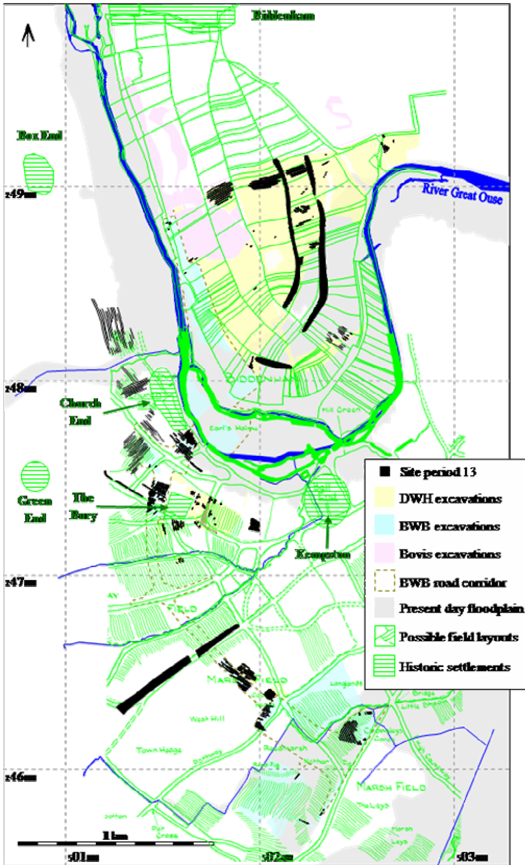
Figure 54: Overall plan of the medieval period SP13 with field layouts reconstructed from historical sources, fieldwork and aerial photographs (Wood 1984).
