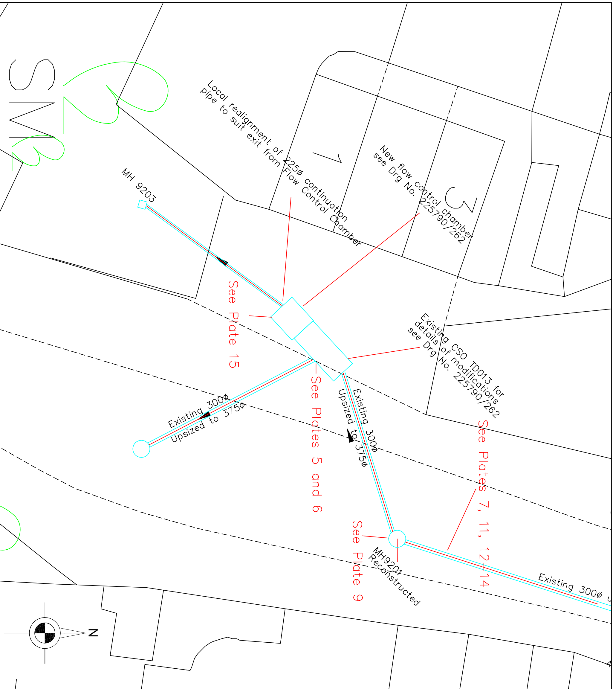
Figure 4 : Corbridge Sewer Refurbishment Works
