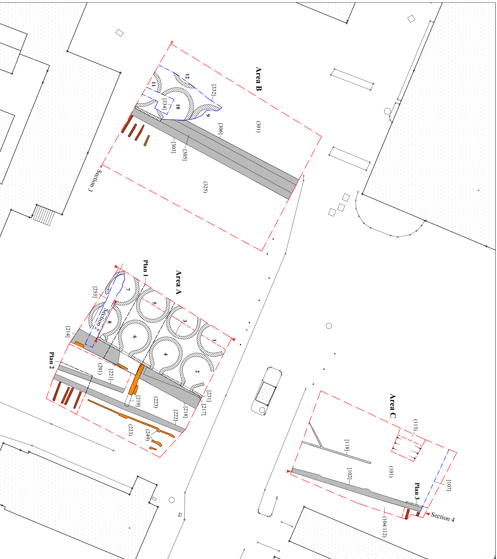
Figure 3 : Location of excavated features and coking ovens (Ovens 1-12)
