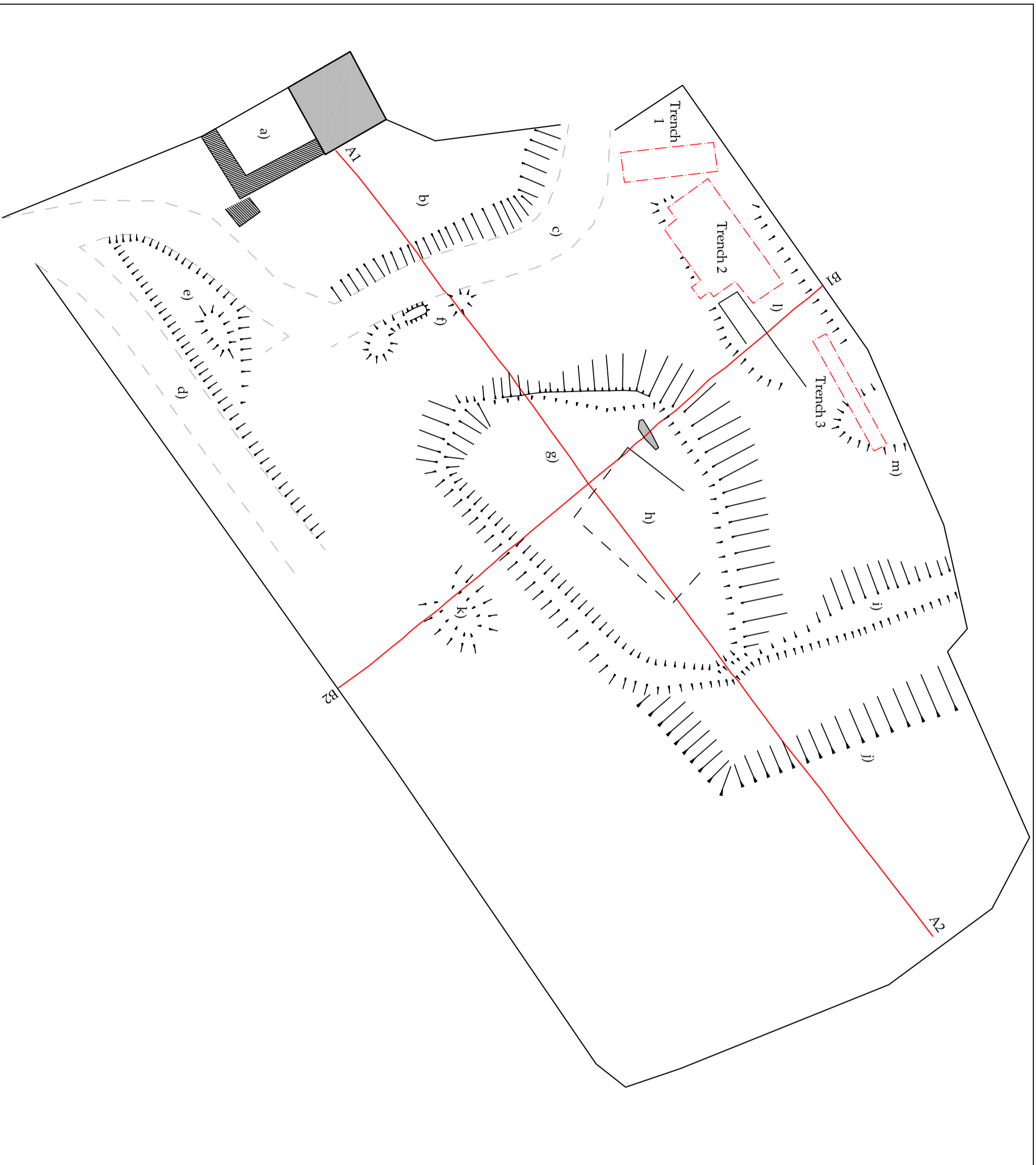
Figure 3 : Plan of features recorded during the topographic survey showing evaluation trench locations (Trenches 1-3)
