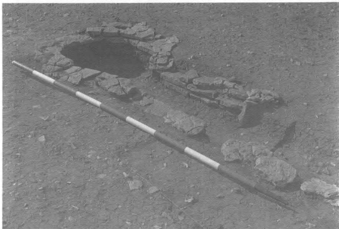
Plate 14: MK301 Stantonbury: Keyhole-shaped oven in Building 1 (photo: MKAU).
