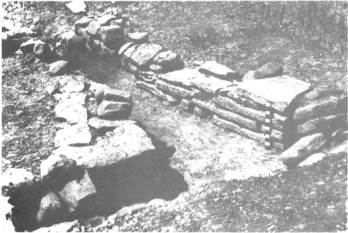
Plate 2: MK96 Windmill Hill: Corn Drier 2 (photo: P. N. Jarvis).
