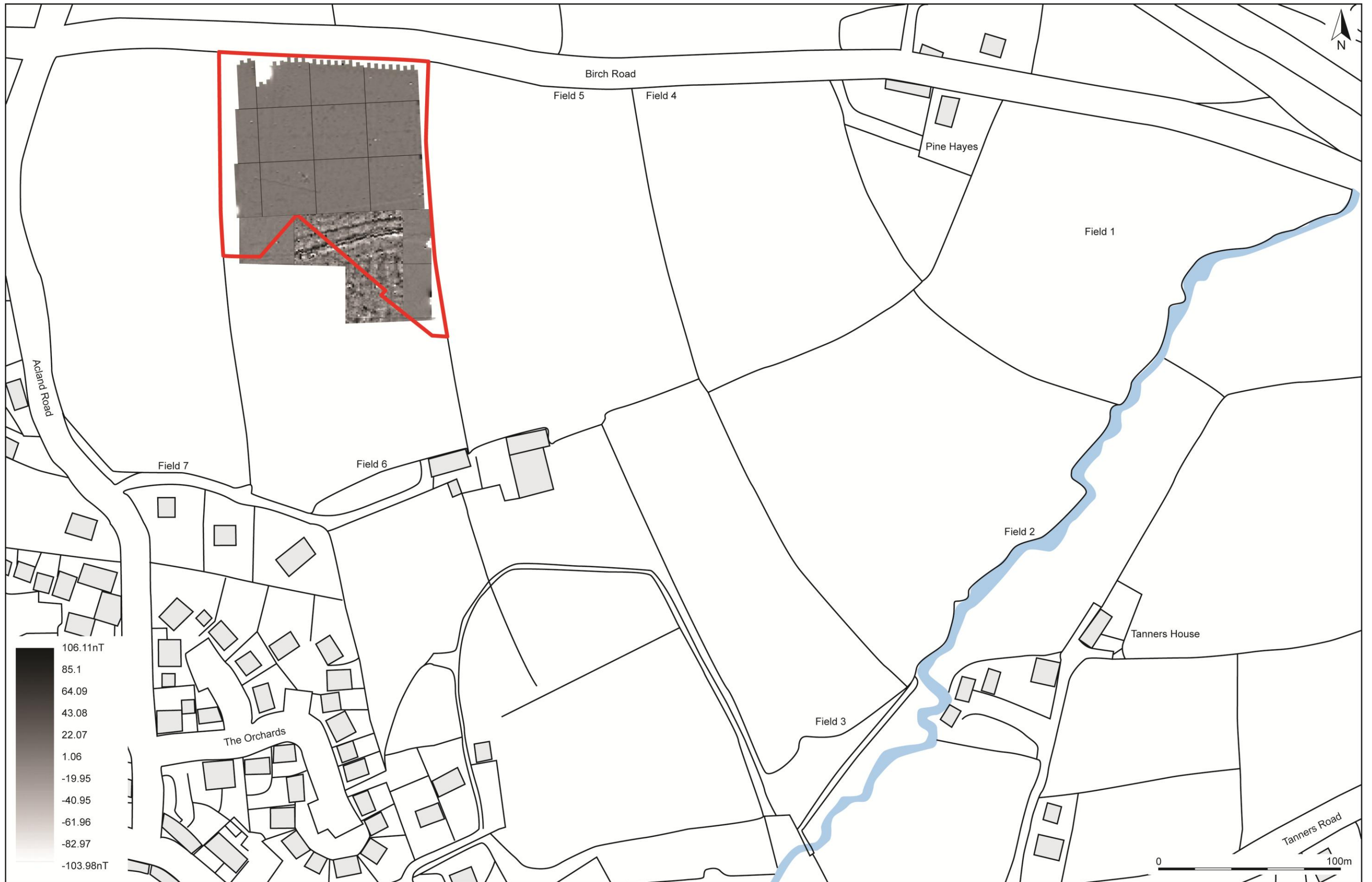
FIGURE 9: GREYSCALE SHADE PLOT OF GRADIOMETER SURVEY DATA (PHASE 1 AND 2); GRADIATED SHADING.
