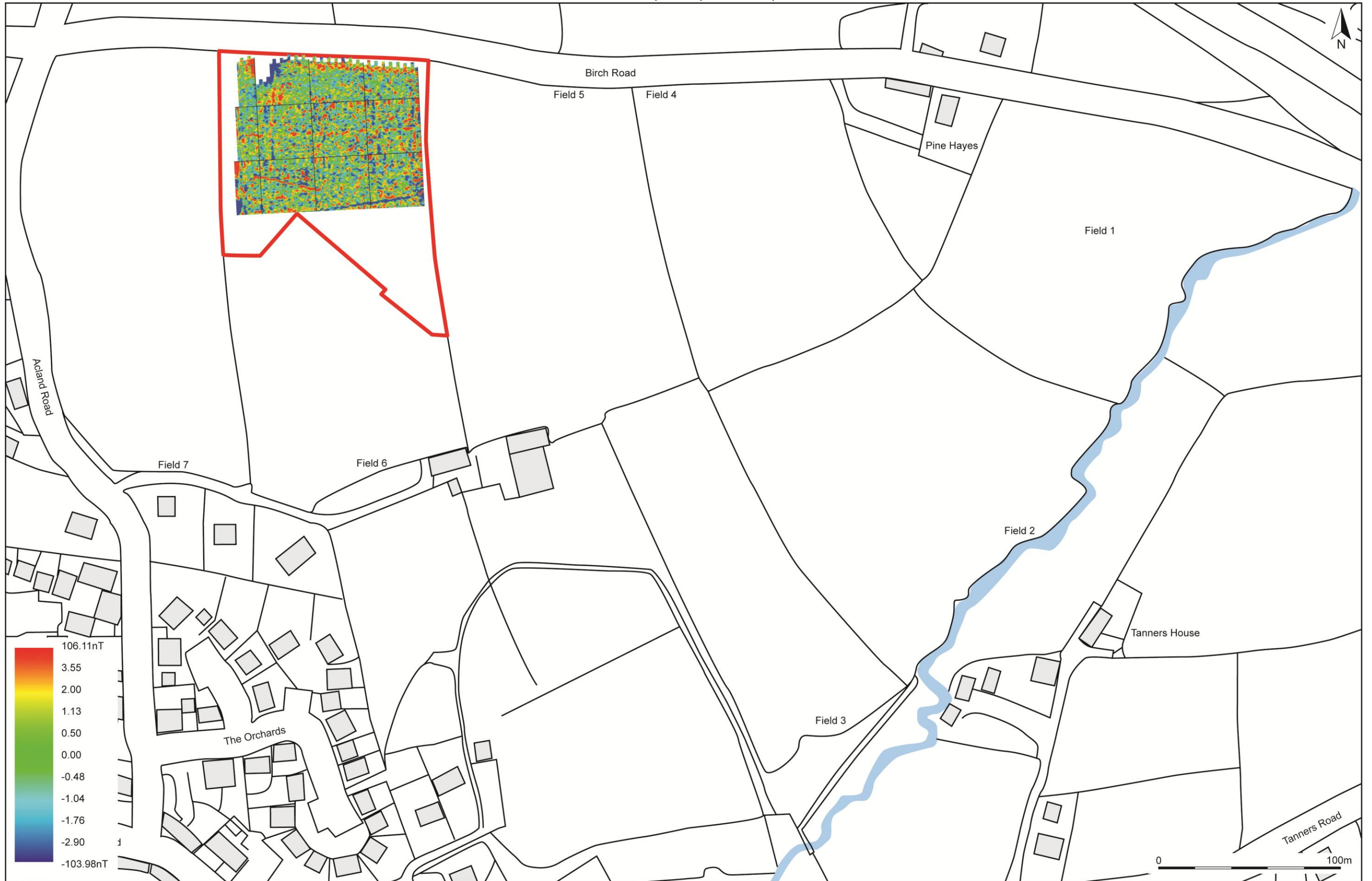
FIGURE 10: RED-BLUE-GREEN (2) SHADE PLOT OF GRADIOMETER SURVEY DATA (PHASE 2 SURVEY DATA ONLY).
