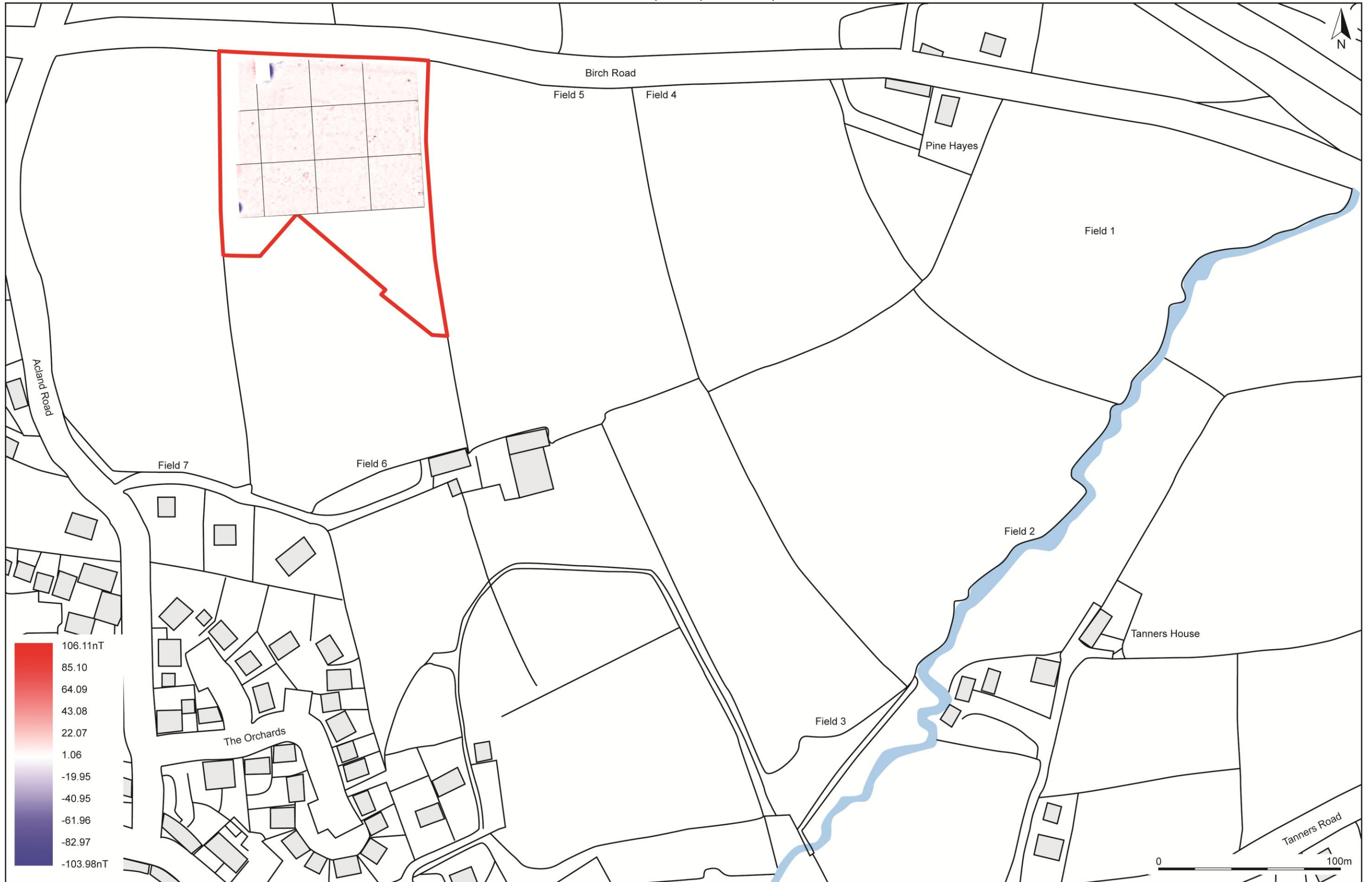
FIGURE 11: RED-WHITE-BLUE SHADE PLOT OF GRADIOMETER SURVEY DATA (PHASE 2 SURVEY DATA ONLY); GRADIATED SHADING.
