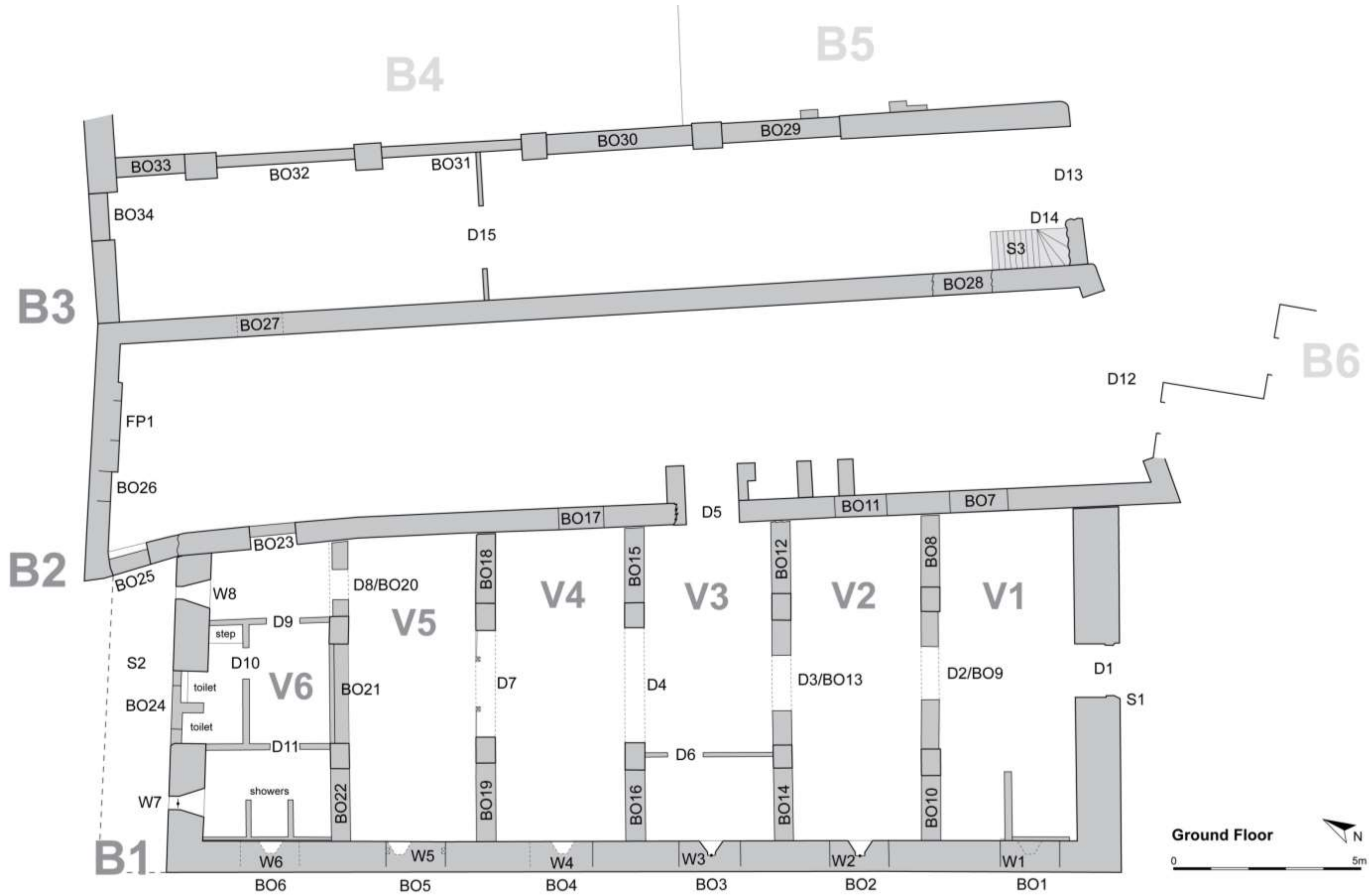
FIGURE 14: GROUND-FLOOR PLAN OF B1-B3 SHOWING DOORS (Dx), WINDOWS (Wx), FIRE PLACES (FPx), BLOCKED OPENINGS (BOx) AND SIGNIFICANT FEATURES (Sx).
