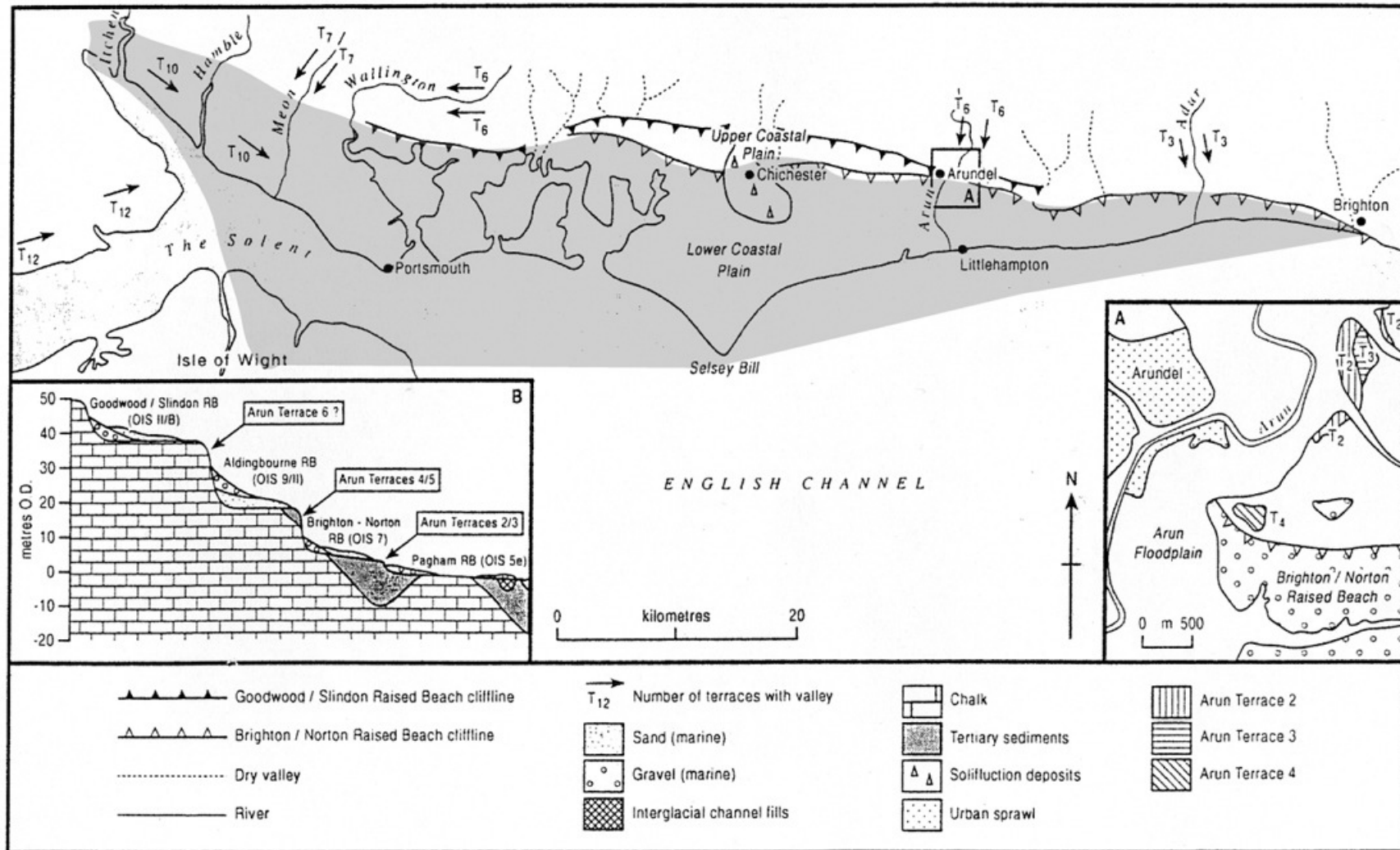
Figure 4. Raised beaches of the West Sussex Coastal Plain.
