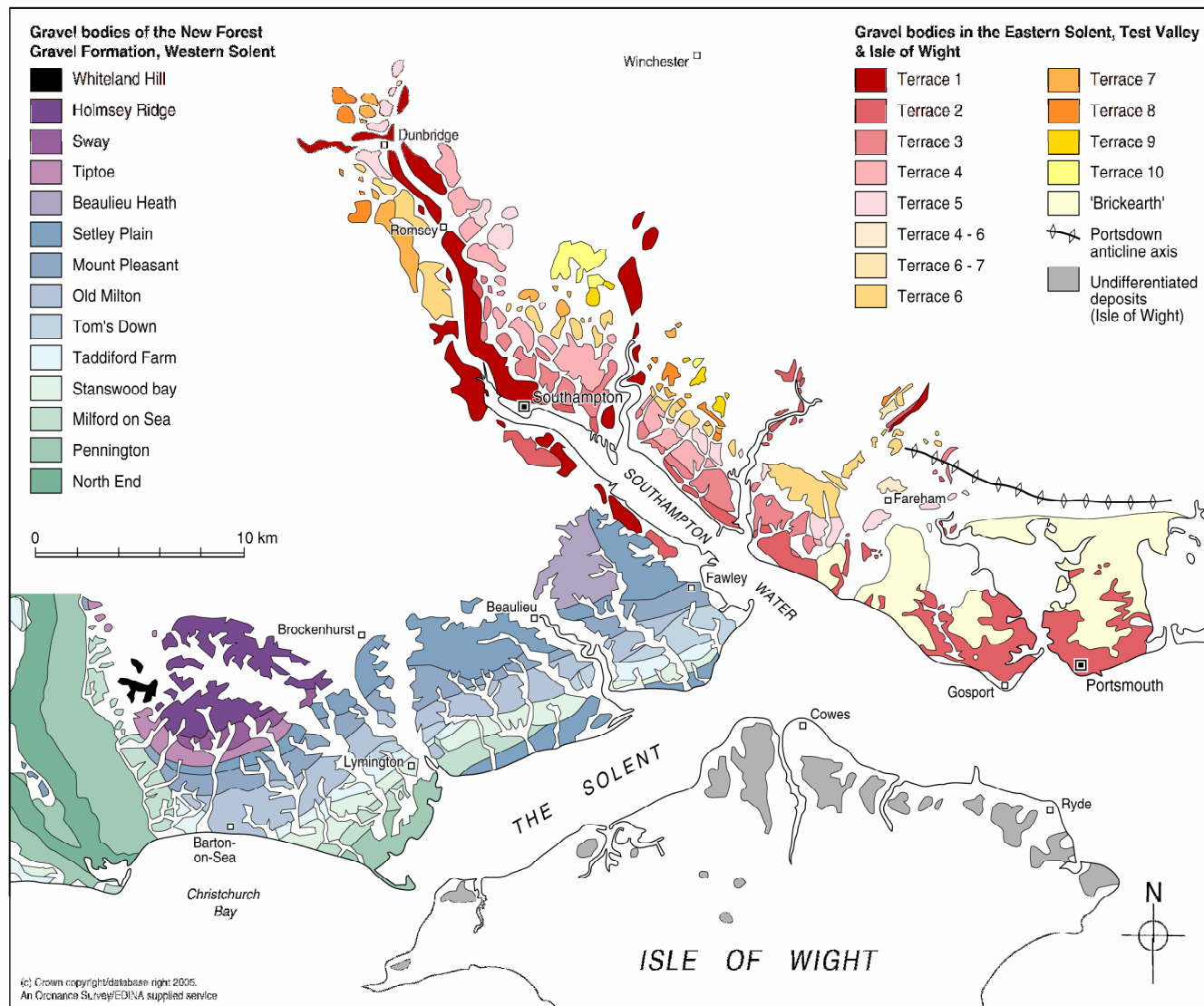
Figure 5. Fluvial deposits of the Solent River system.
