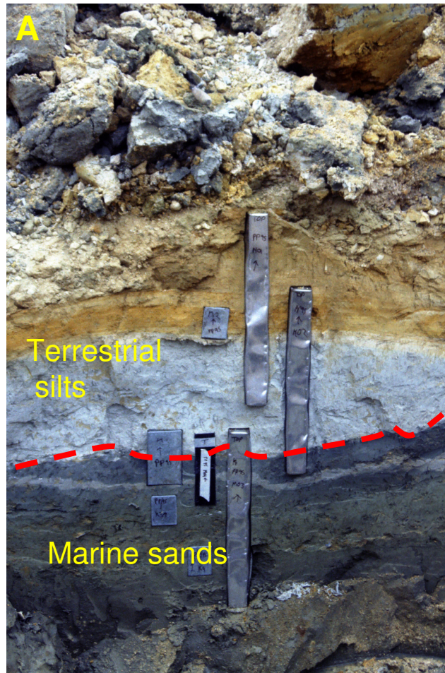
Figure 8. Portfield Pit, Westhampnett. A. Marine and terrestrial sediments above and below old landsurface. B. Animal bones weathered out of old landsurface. C. Peat accumulating in channel cut through old landsurface and into underlying marine sands.
