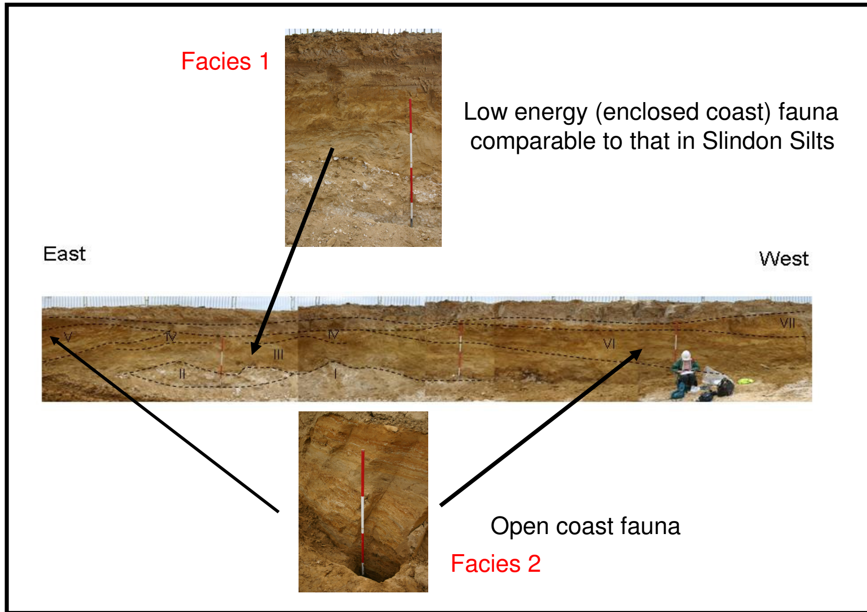
Figure 9. Complex stratigraphy from the Aldingbourne Raised Beach at Pear Tree Knap.
