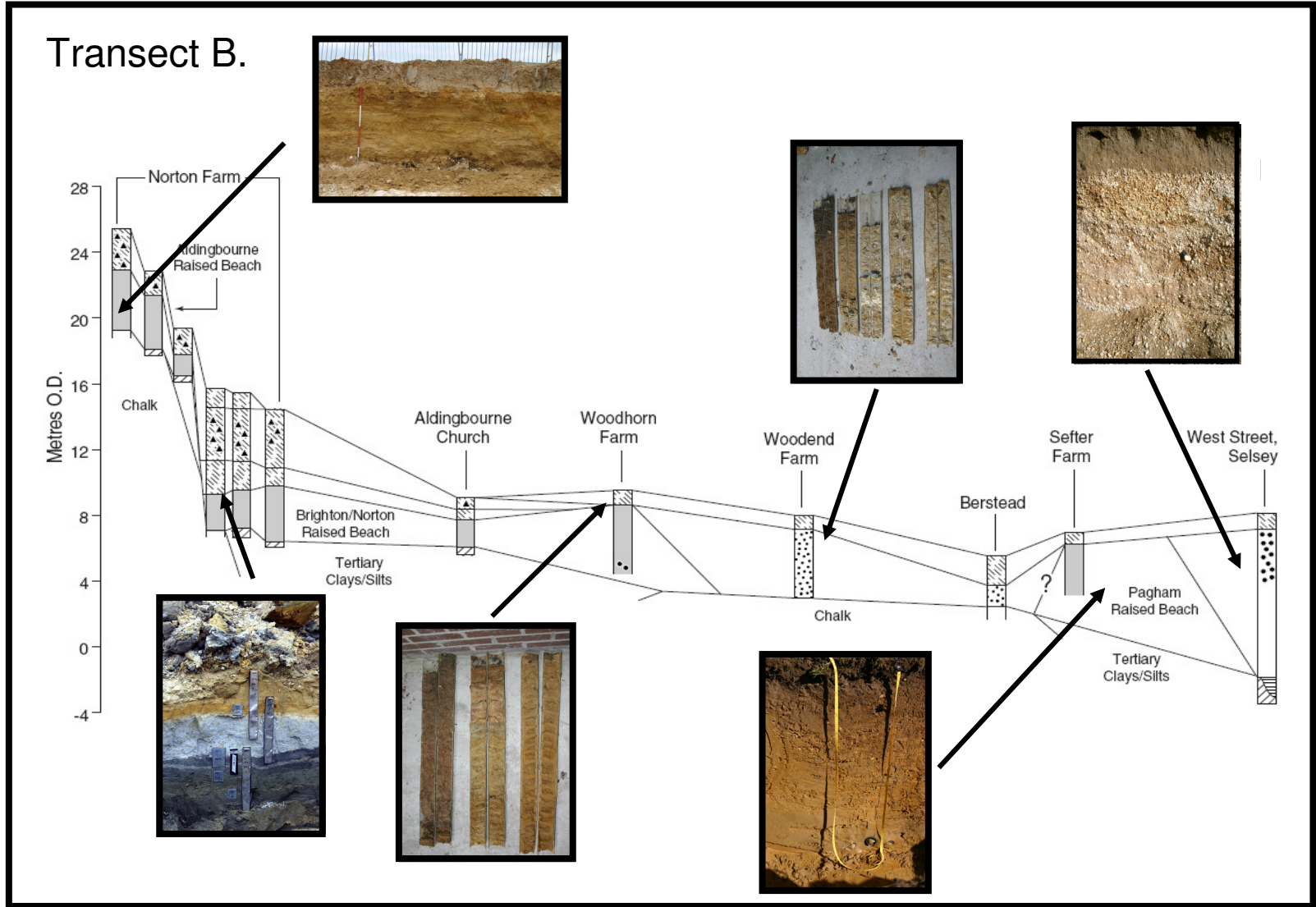
Figure 10. Transect through Lower Coastal Plain east of Chichester showing elements of the Aldingbourne, Brighton/Norton and Pagham Raised Beaches as well as the Woodend Silts.
