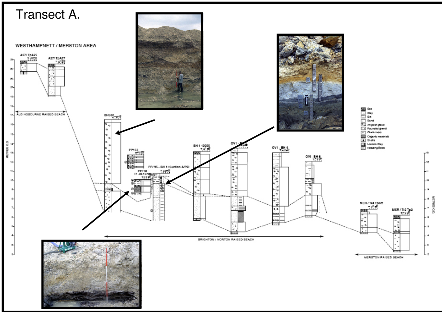
Figure 16. Transect through sediments east of Chichester.
