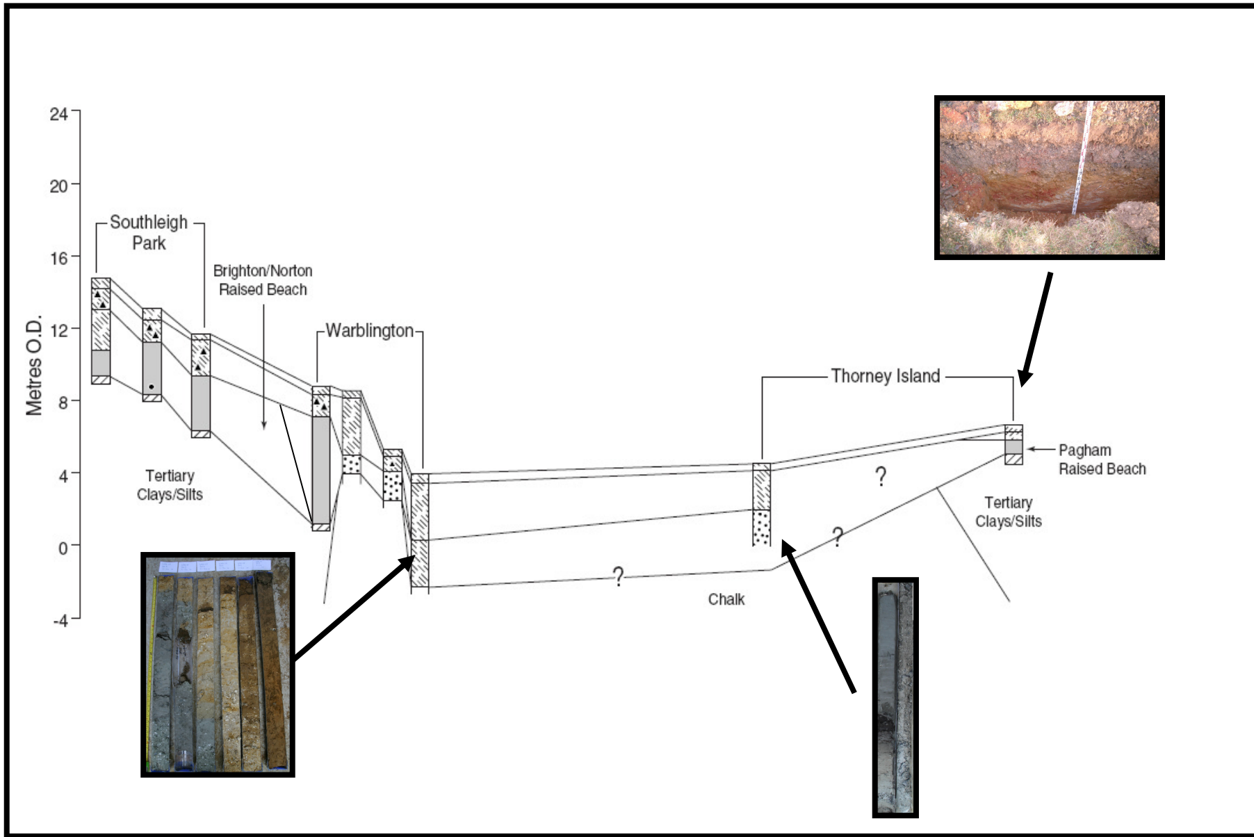
Figure 18. Stratigraphic section in the Havant/Thorney Island area showing the Warblington area.
