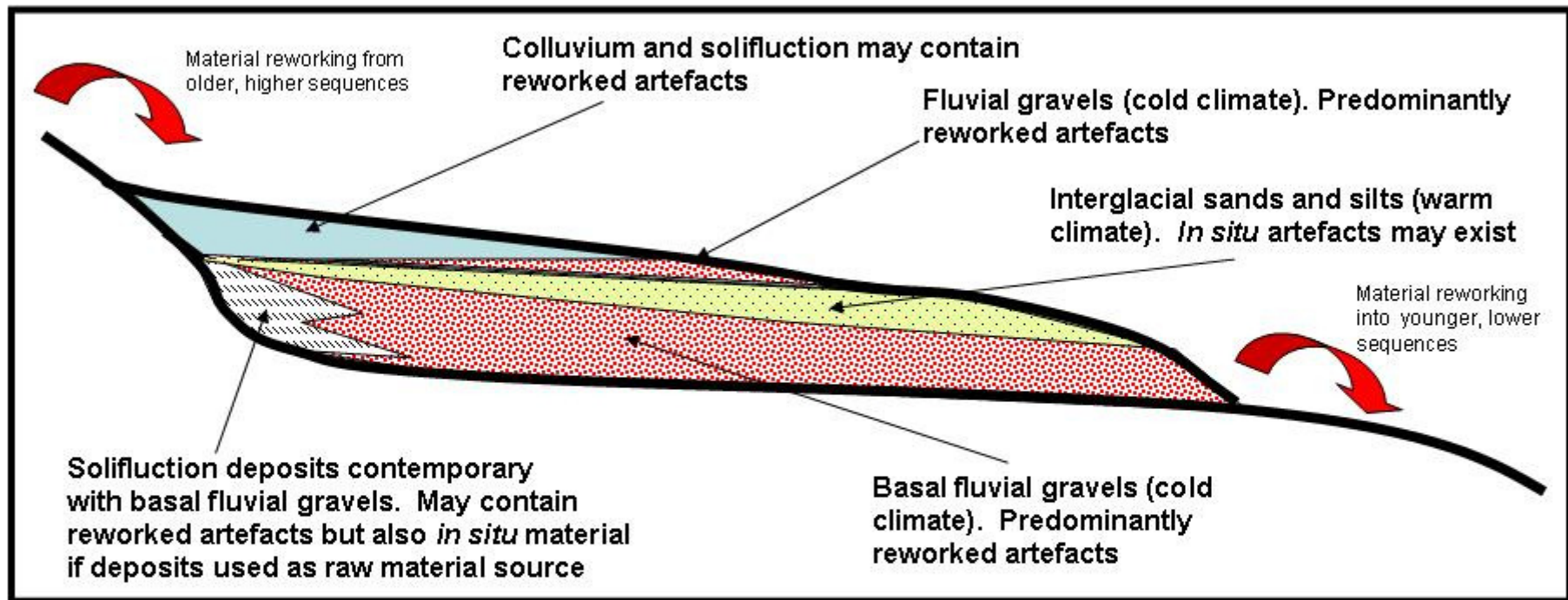
Figure 31. A geoaerchaeological model for Palaeolithic artefacts within a fluvial sequence beneath a terrace.
