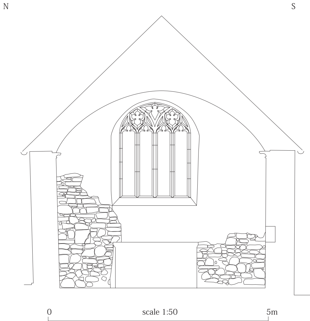
Fig. 11 Internal East elevation showing exposed stones plotted by corrected photography.
