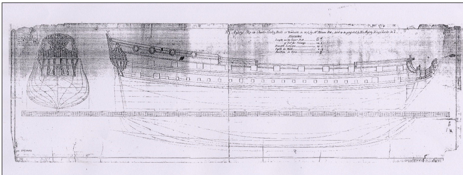
Fig 65 'Lines' plan of the Charles Galley (National Maritime Museum)
