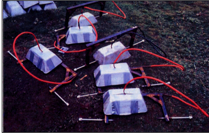
Fig 59 Zinc anodes deployed on the cannon and anchor at the wreck of the Swan at Duart Point, Scotland
