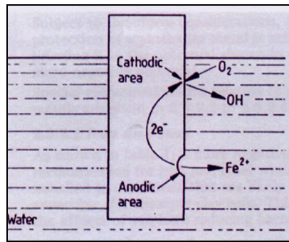
Fig 50 Anodic and cathodic reactions at metal surface in oxygenated and aqueous conditions (after British Standards Institute 1991)
