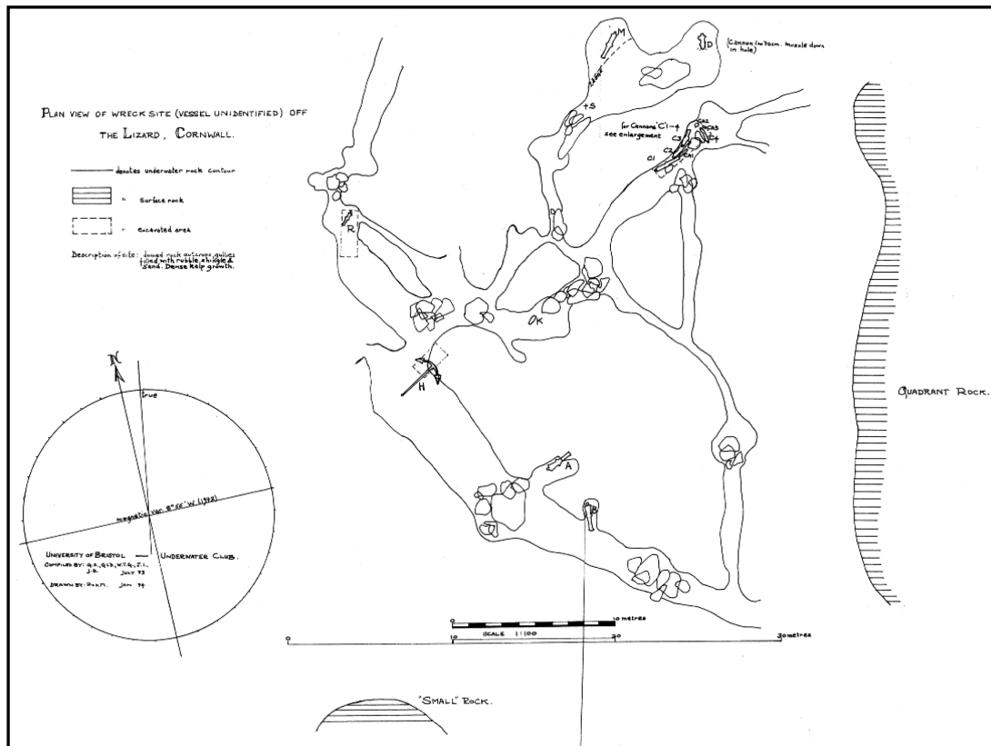
Fig 19 Quadrant Rock site plan, probably drawn by UBUC c1973
