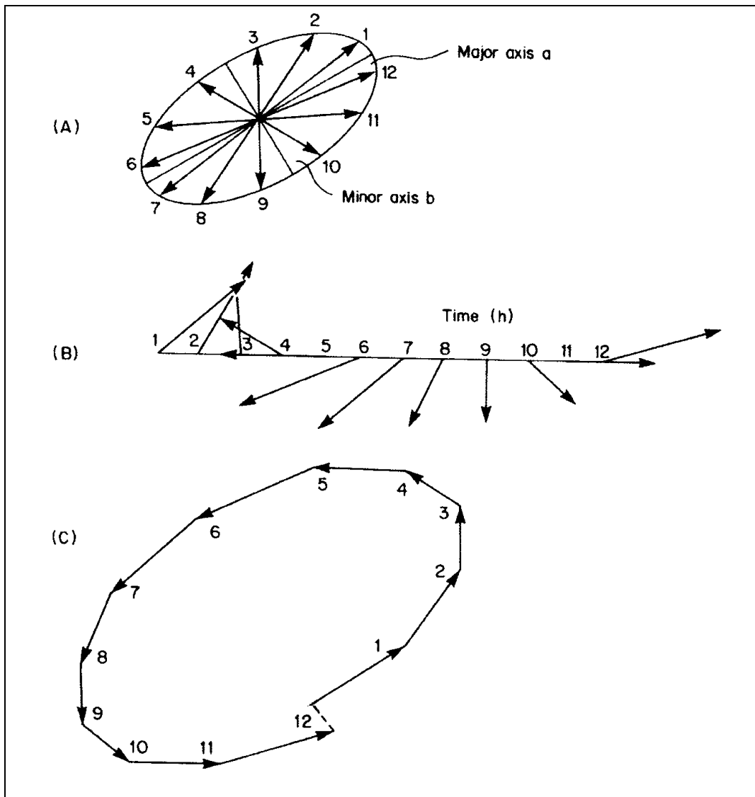
Fig 38 Tidal current vectors (from Dyer 1986)
