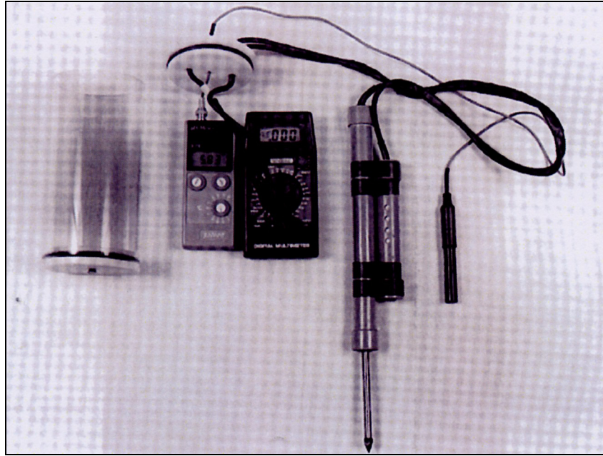
Fig 55 Equipment for determining surface pH and E_{corr} , showing from left to right: polycarbonate waterproof housing with o-ring seal, pH meter, high impedance multi-meter, working electrode (AISI 316 stainless steel) with attached reference electrode, and flat surface pH electrode. (© National Museum of Denmark)
