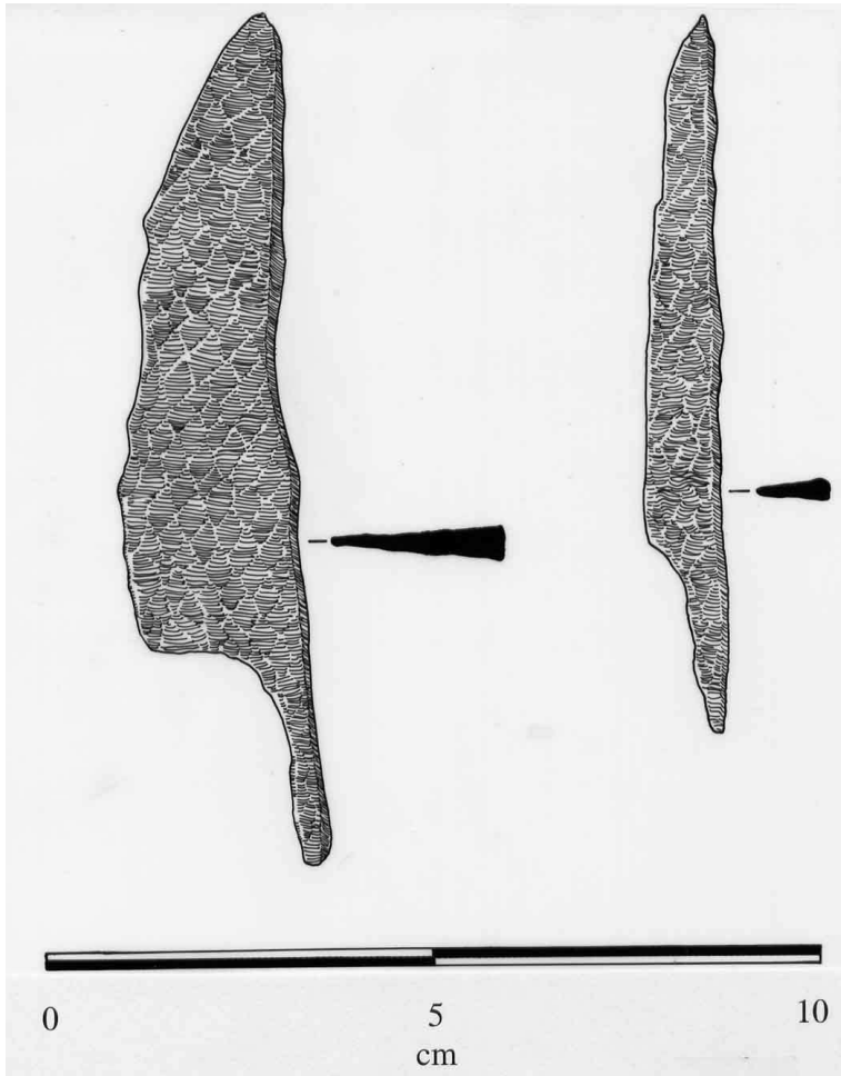
A3.1: Iron knives 2.13 and 2.28, recovered from Danebury used as prototypes for the experimental tools. Source: Cunliffe, 1984: 350.
