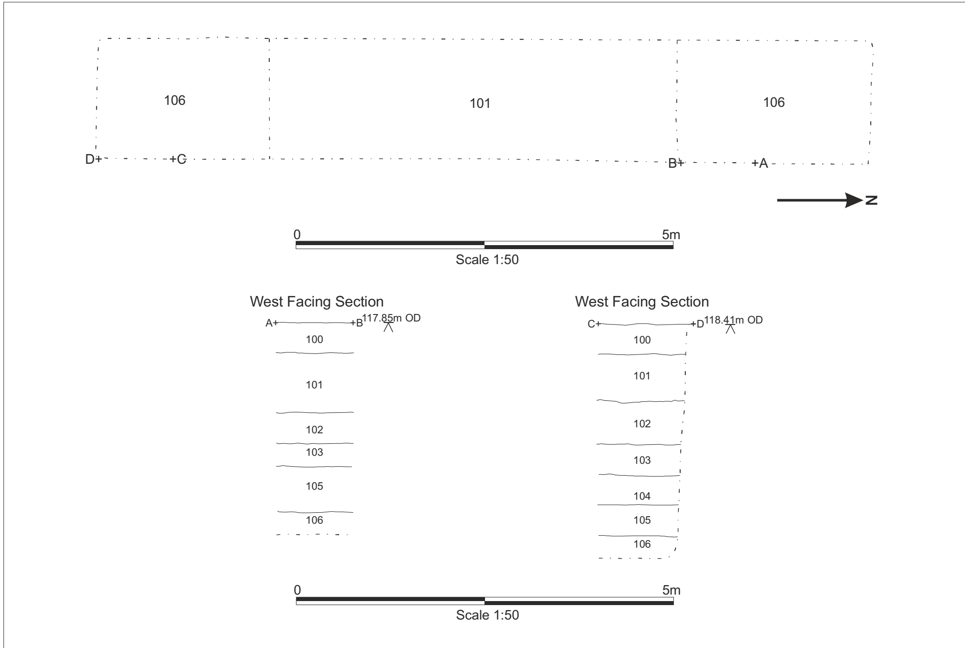
Figure 3: Trench 1 plan and sections at scale 1:50
