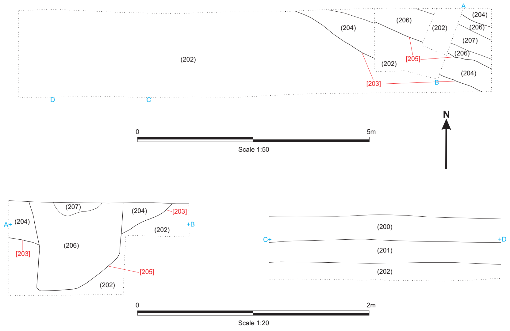
Figure 4: Trench 2 plan and sections (scales 1:50 and 1:20)
