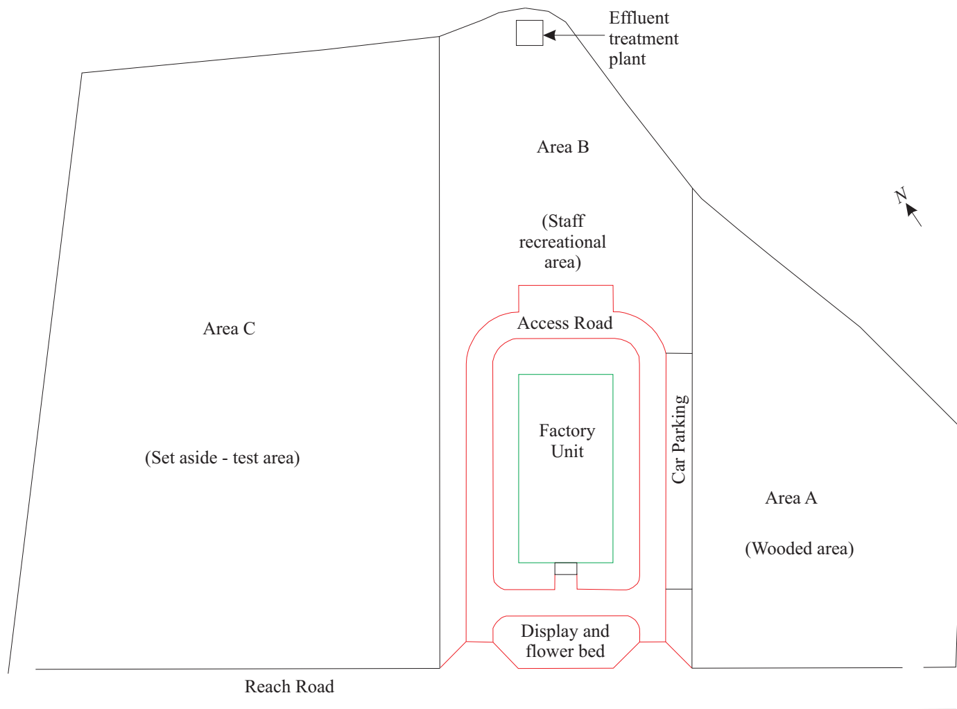
Figure 2: Development proposal at scale 1:1000
