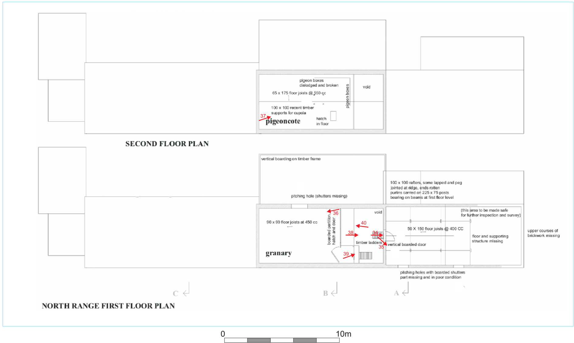
Figure 4: Plans of the first and second floors of the north range, as existing, with the plate number and position of photographs shown in red (listed in appendix 1) (scale 1:200).
