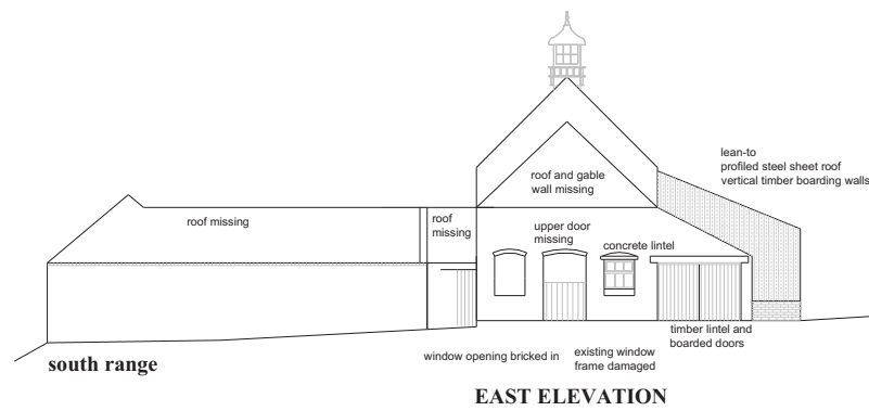
EAST ELEVATION
