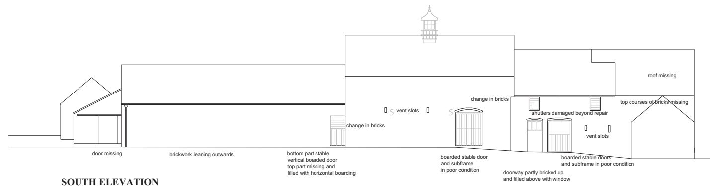
SOUTH ELEVATION
