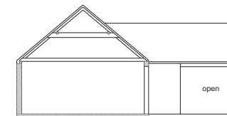
SECTION CC and EAST ELEVATION of west end
