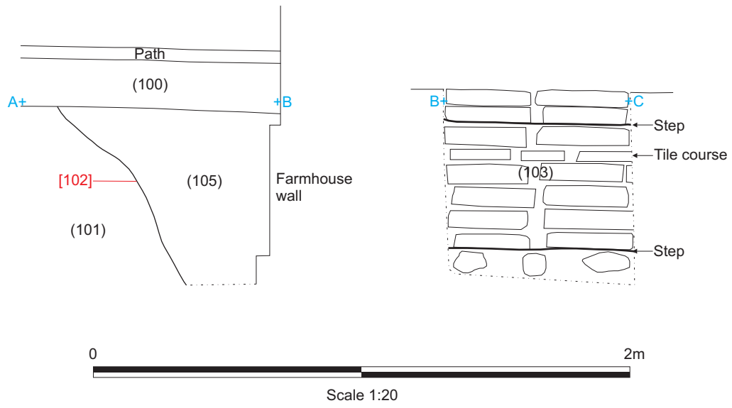
Figure 3: Sections A-B and B-C, south side of the existing farm house (scale 1:20)
