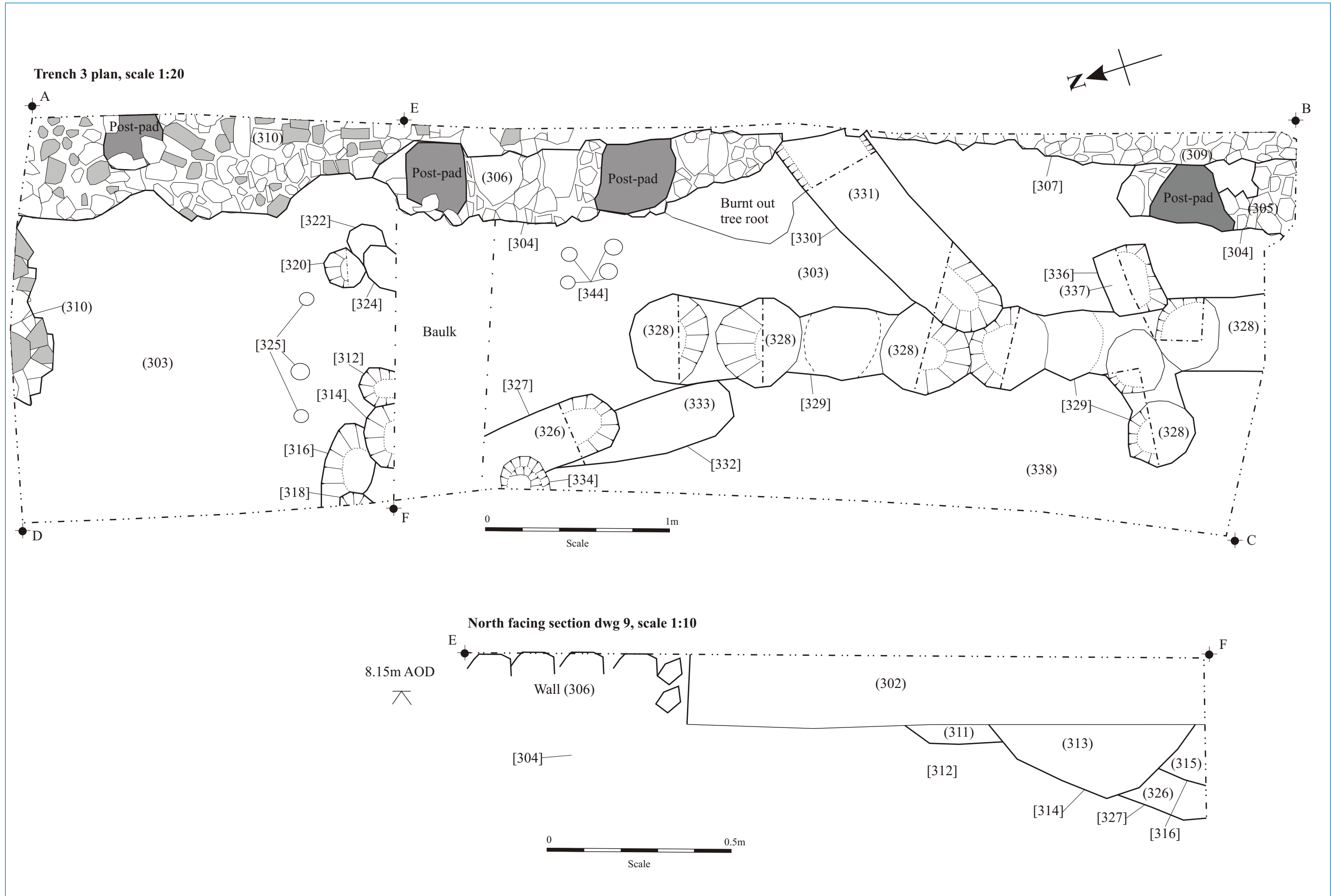
Figure 5: Plan of trench 3 scale 1:20 and section drawing 9 at scale 1:10
