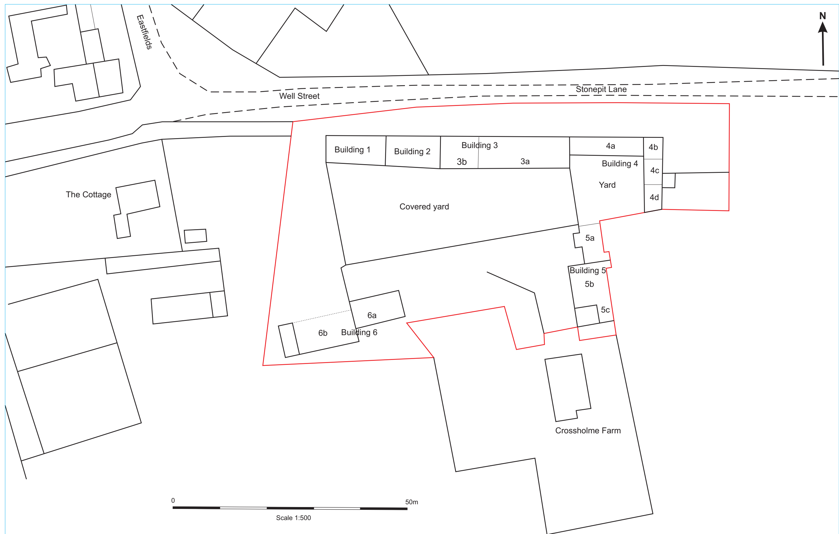
Figure 2: Site location plan at scale 1:500, with the development area outlined in red
