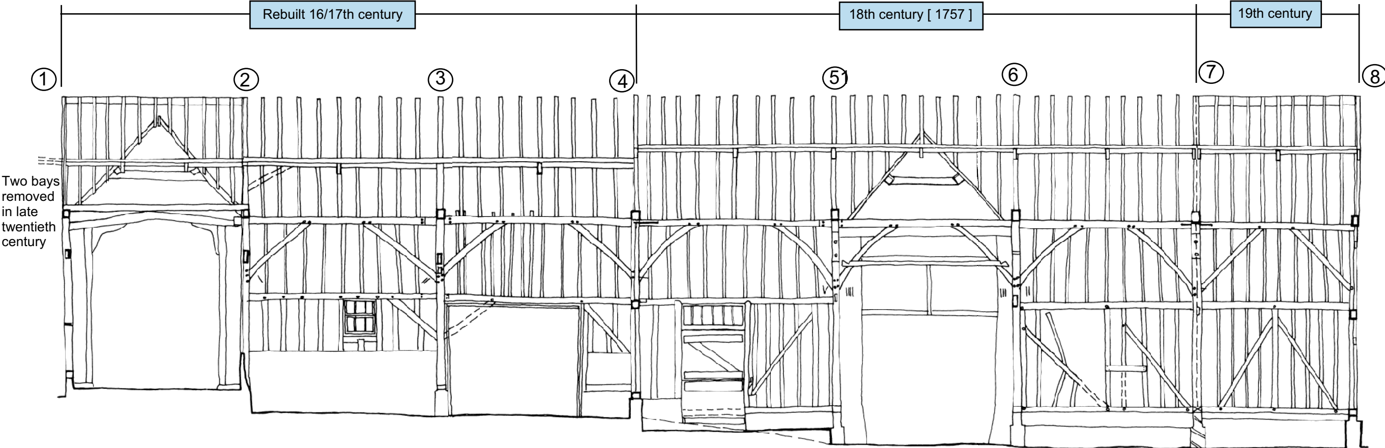
Reduced long section of the west wall showing full length of barn
