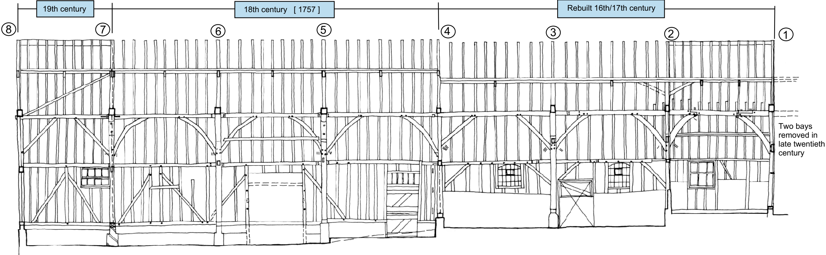
Reduced long section of the east wall showing full length of barn
