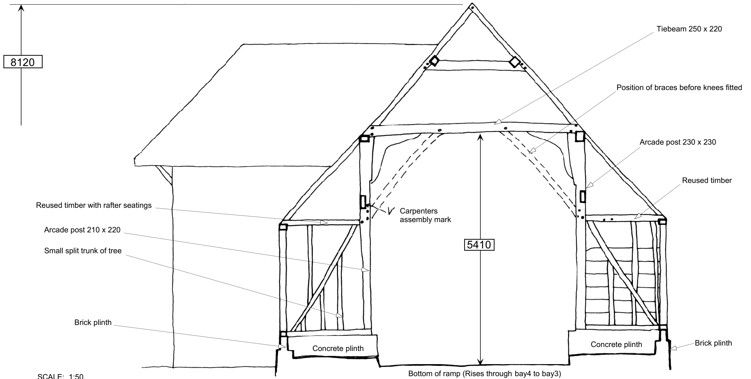
Truss 5 from south and aisle frame on plinth wall. Bay 4 A-F
