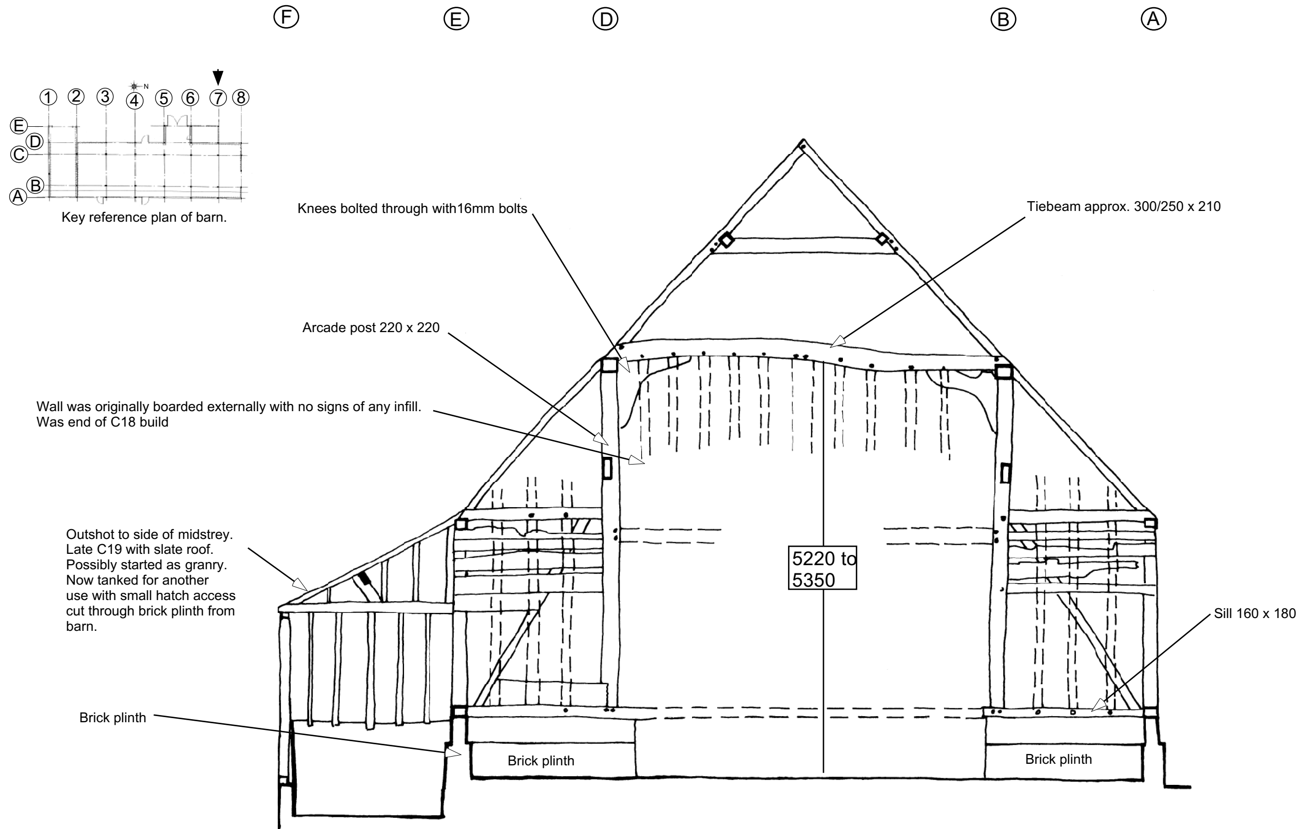
Truss 7 from south and aisle frame on plinth wall. Bay 6 A-E & F to outshot
