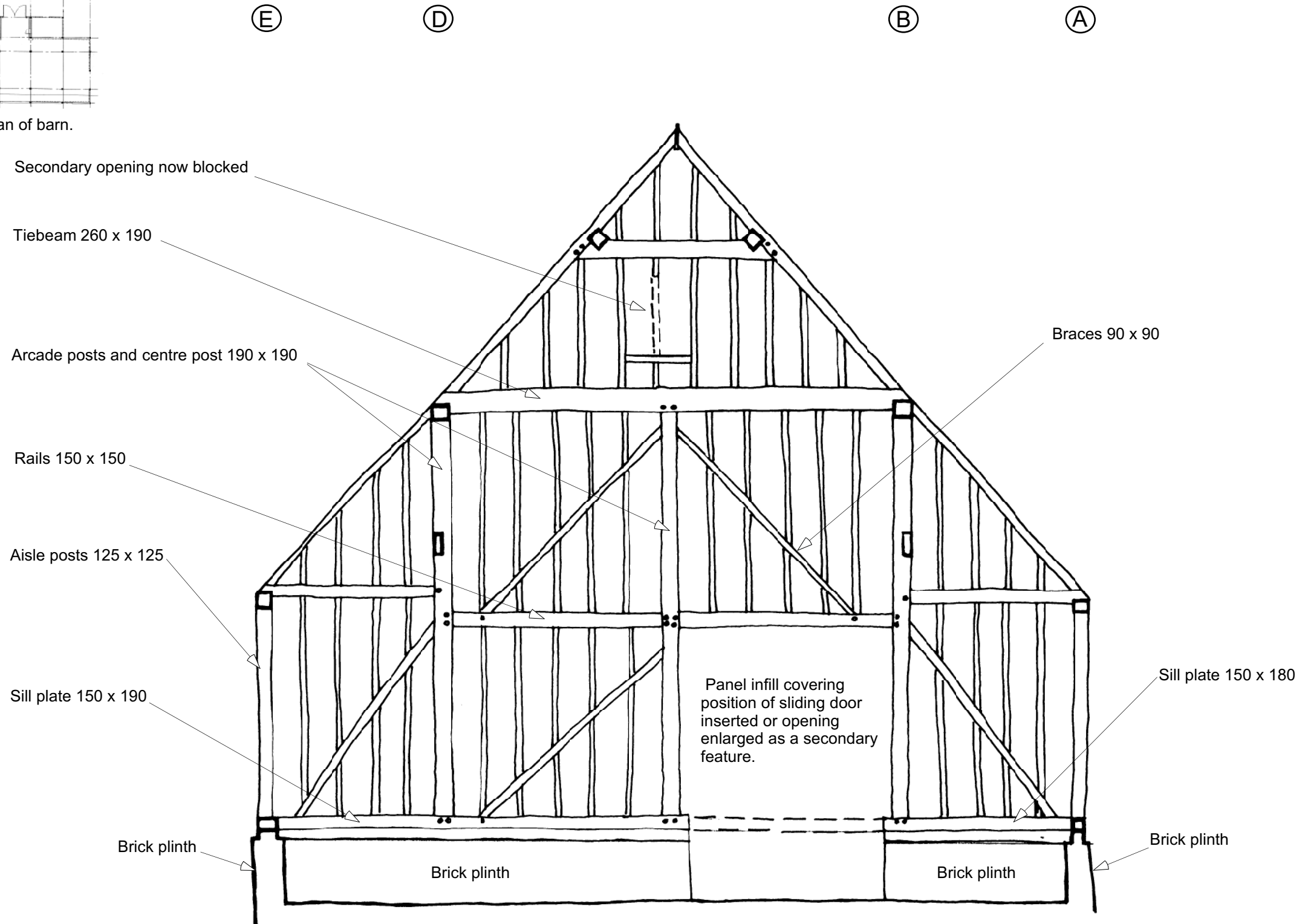
Truss 8 gable wall from south and inside. Bay 7 A-E
