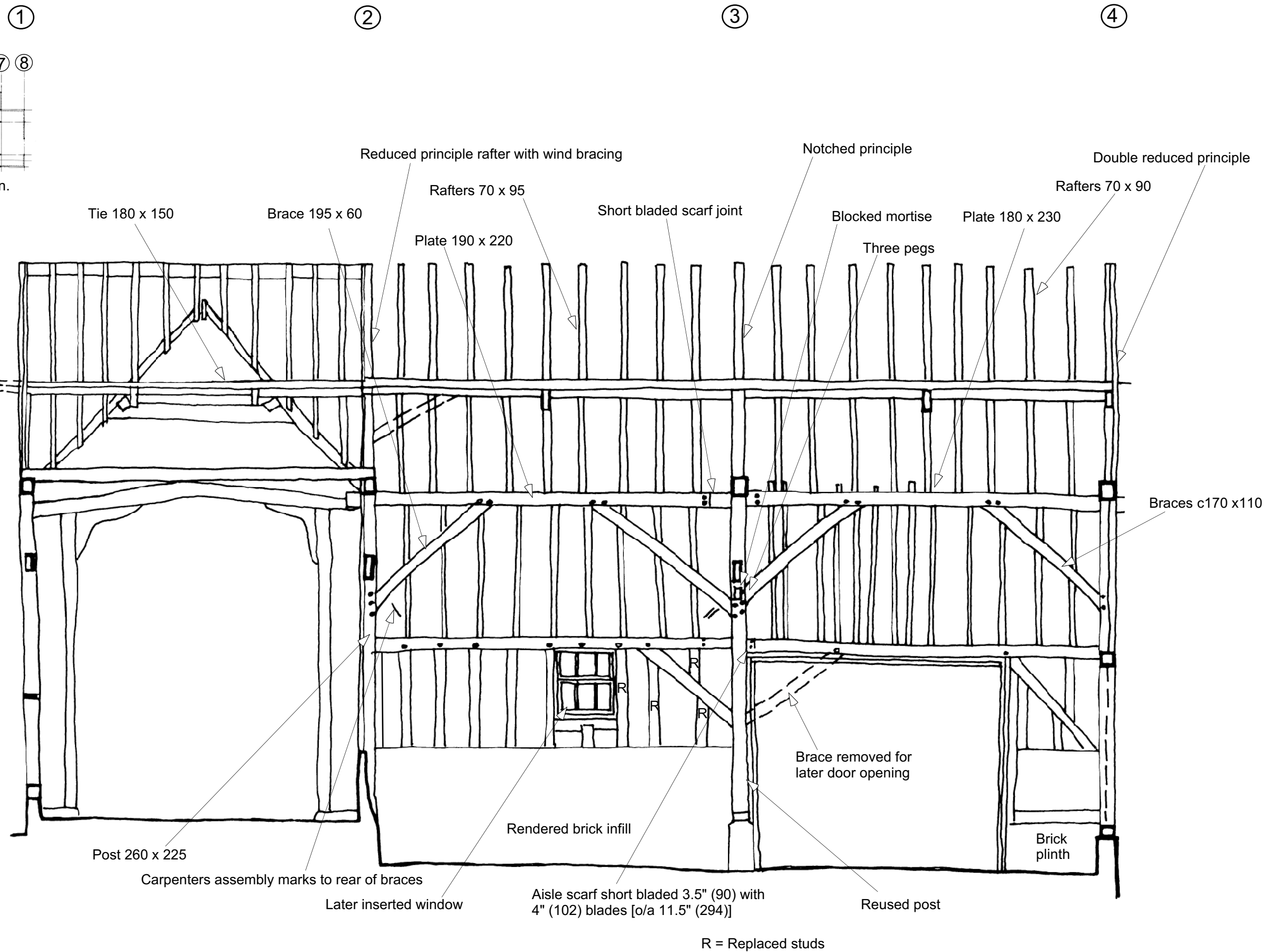
Long section west wall inside bays 1-3
