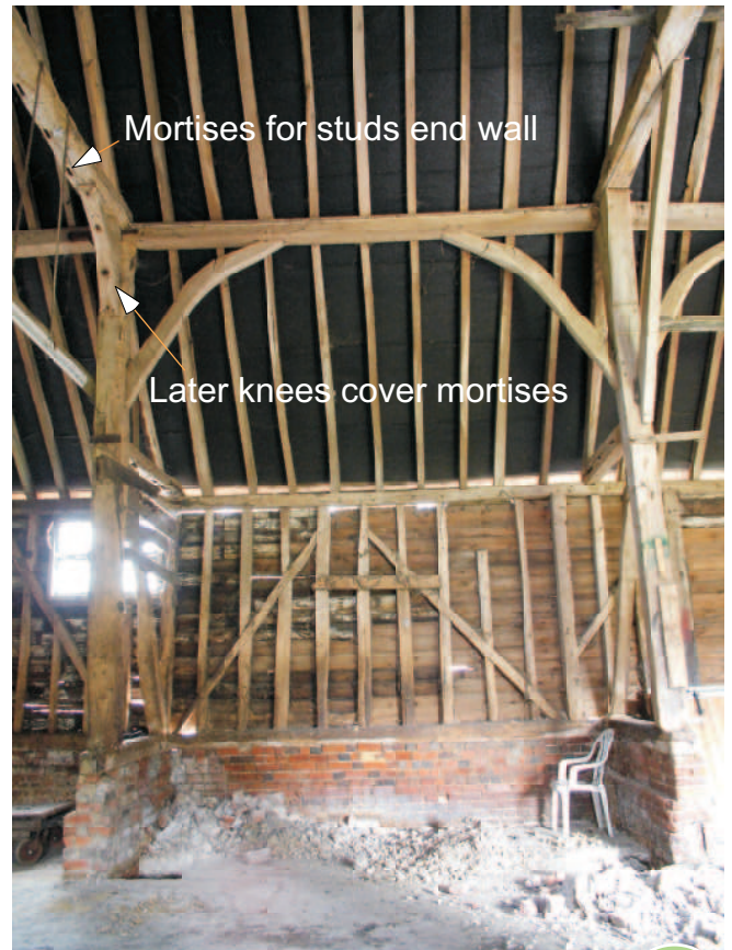
(267) Aisle wall structure bay 6-7. Truss 7 (left) was end this build
