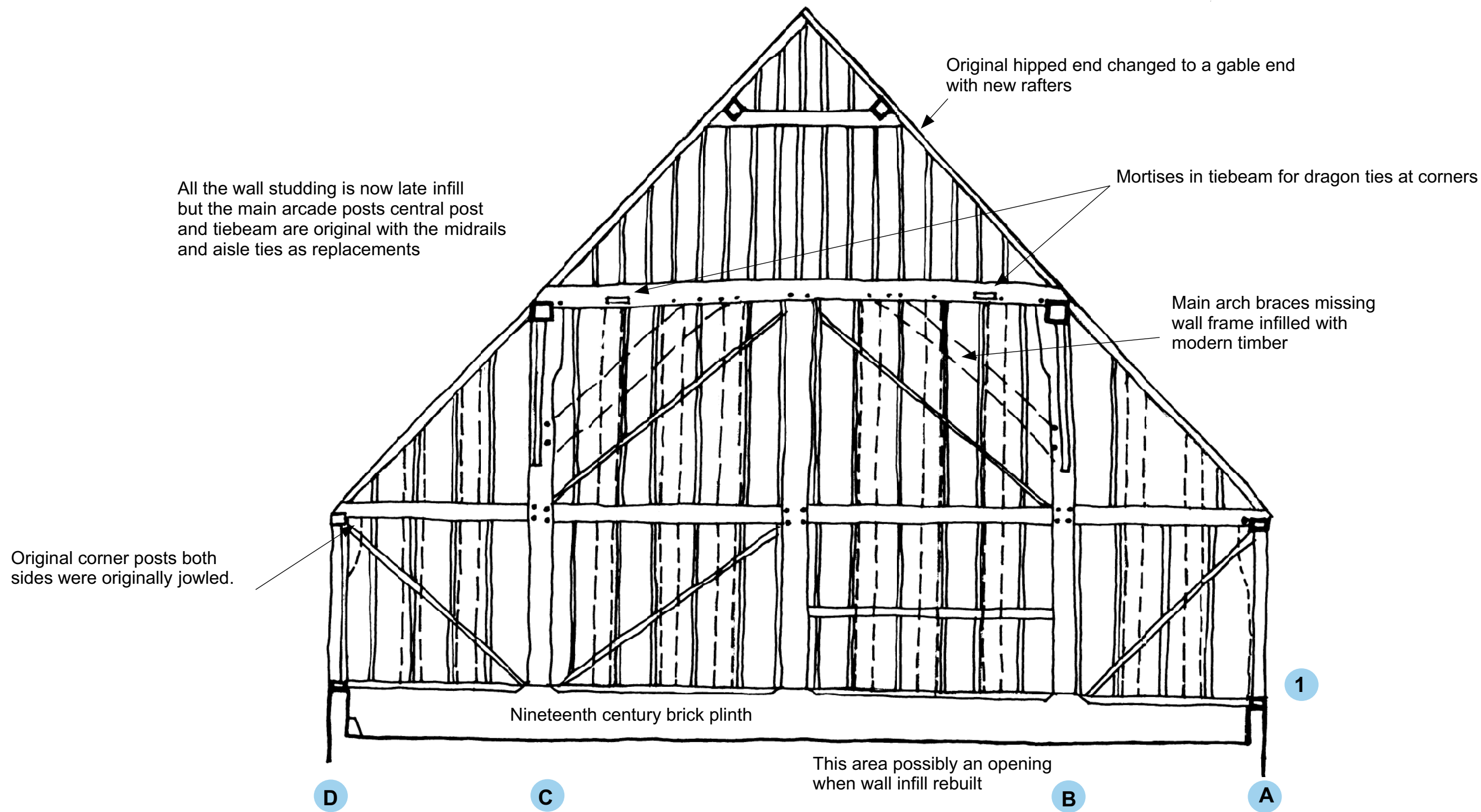
TRUSS 1 A - D SOUTH EAST END OF BARN (Section G on architects drawing)
